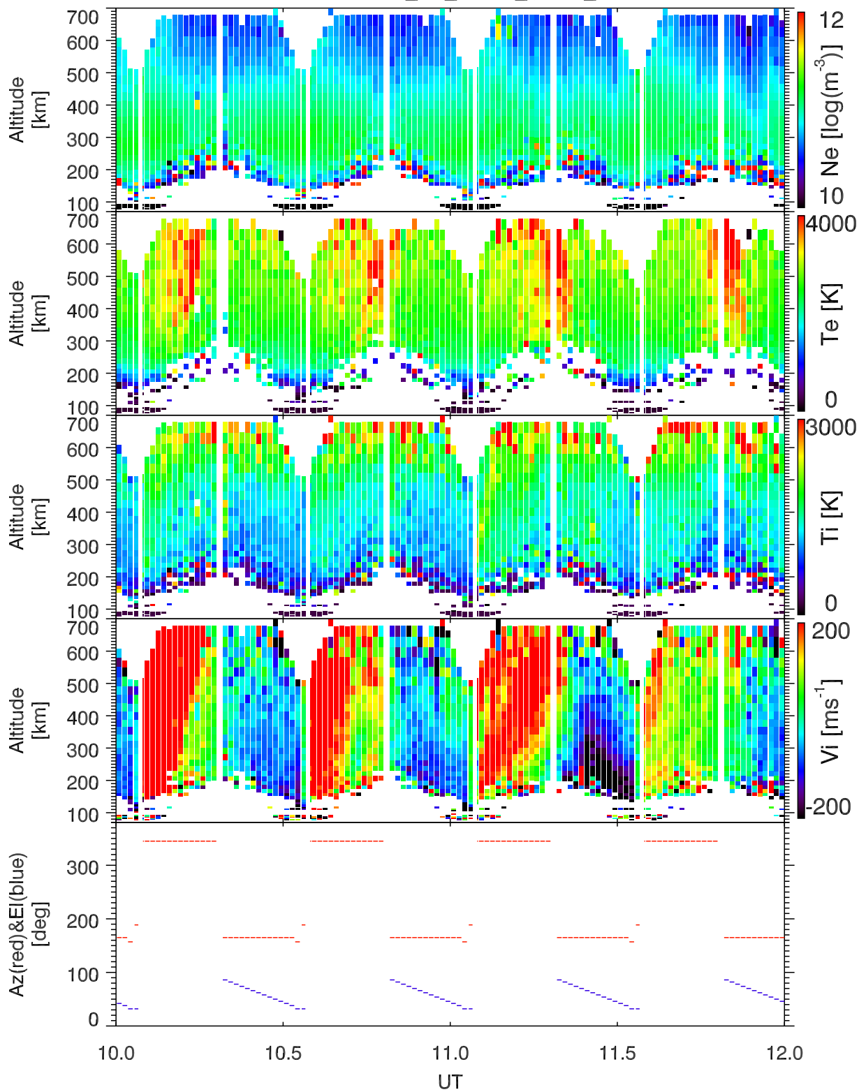
EISCAT 1998-04-29_10_12UT_gup0_ant@32m.
