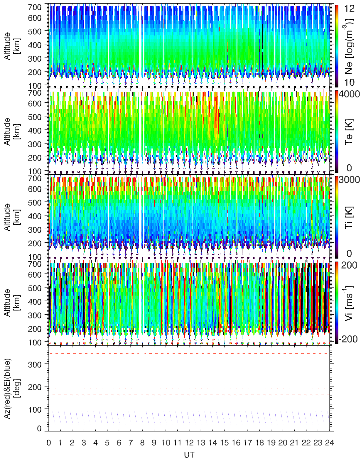
EISCAT 1998-04-30_00_24UT_gup0_ant@32m.
