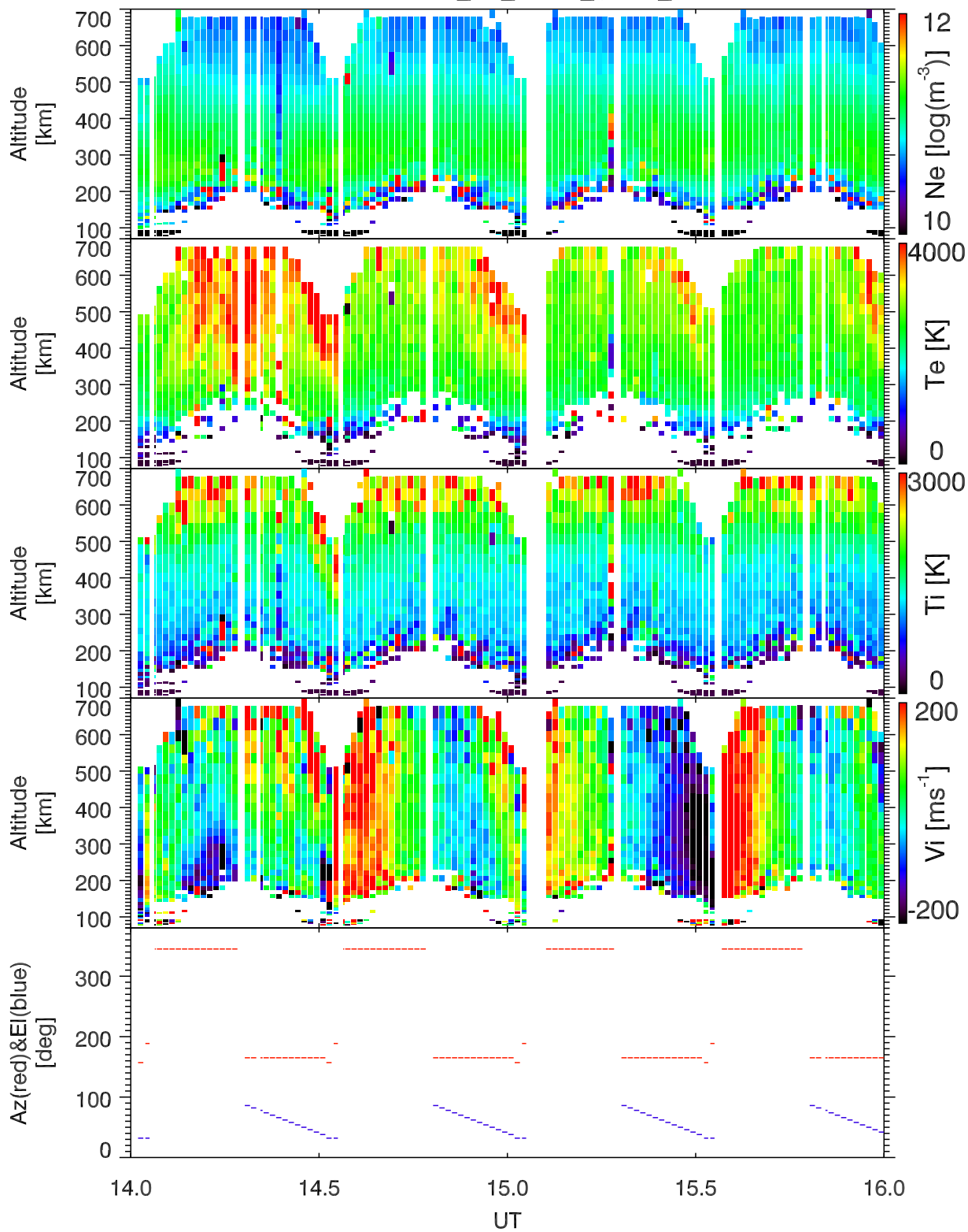
EISCAT 1998-04-30_14_16UT_gup0_ant@32m.
