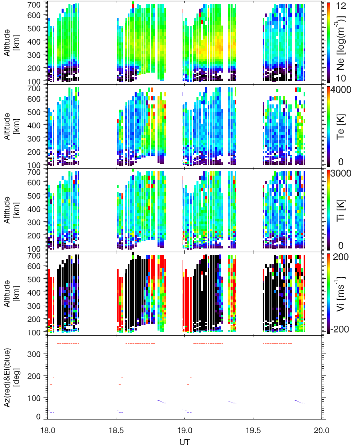
EISCAT 1998-10-20_18_20UT_gup3c_ant@32m.
