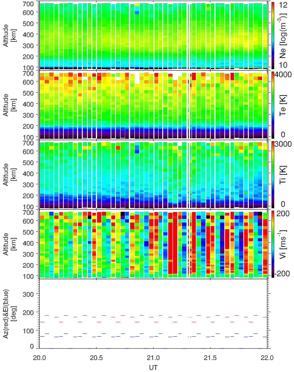
EISCAT 1999-07-01_20_22UT_gup3c_ant@32m.
