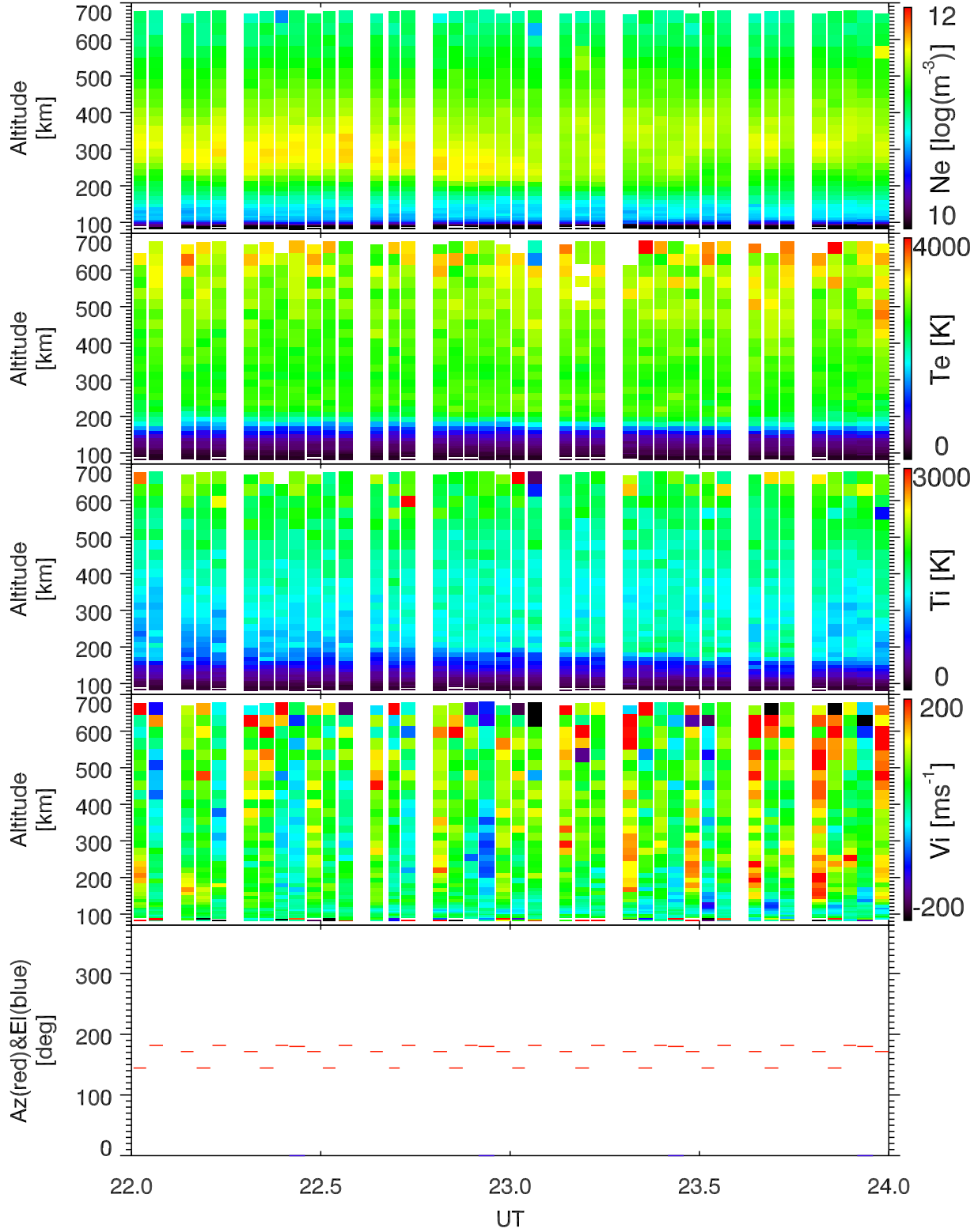
EISCAT 1999-07-05_22_24UT_gup3c_ant@32m.
