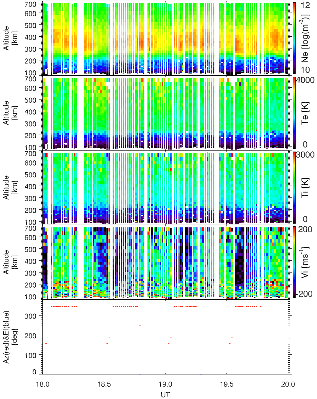
EISCAT 2000-04-12_18_20UT_tau0_ant@32m.
