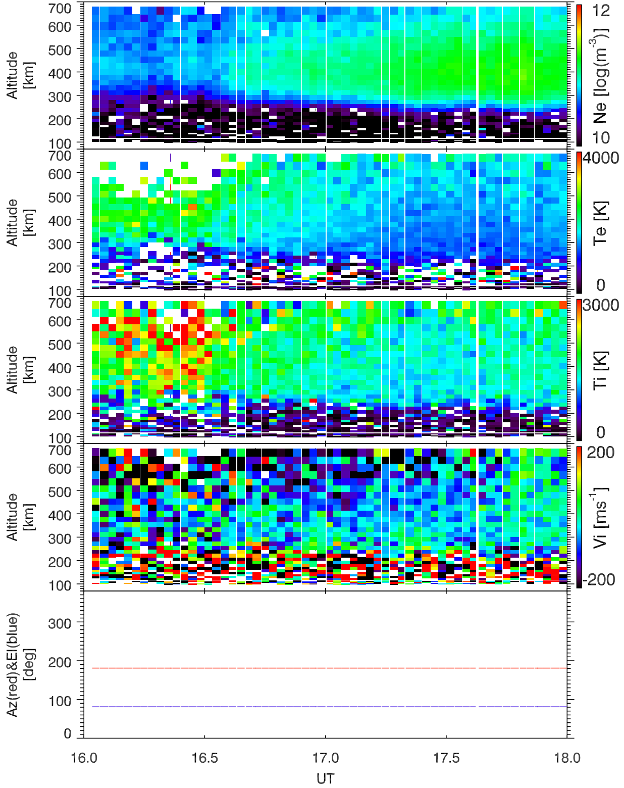
EISCAT 2001-01-21_16_18UT_tau0_all@42m.
