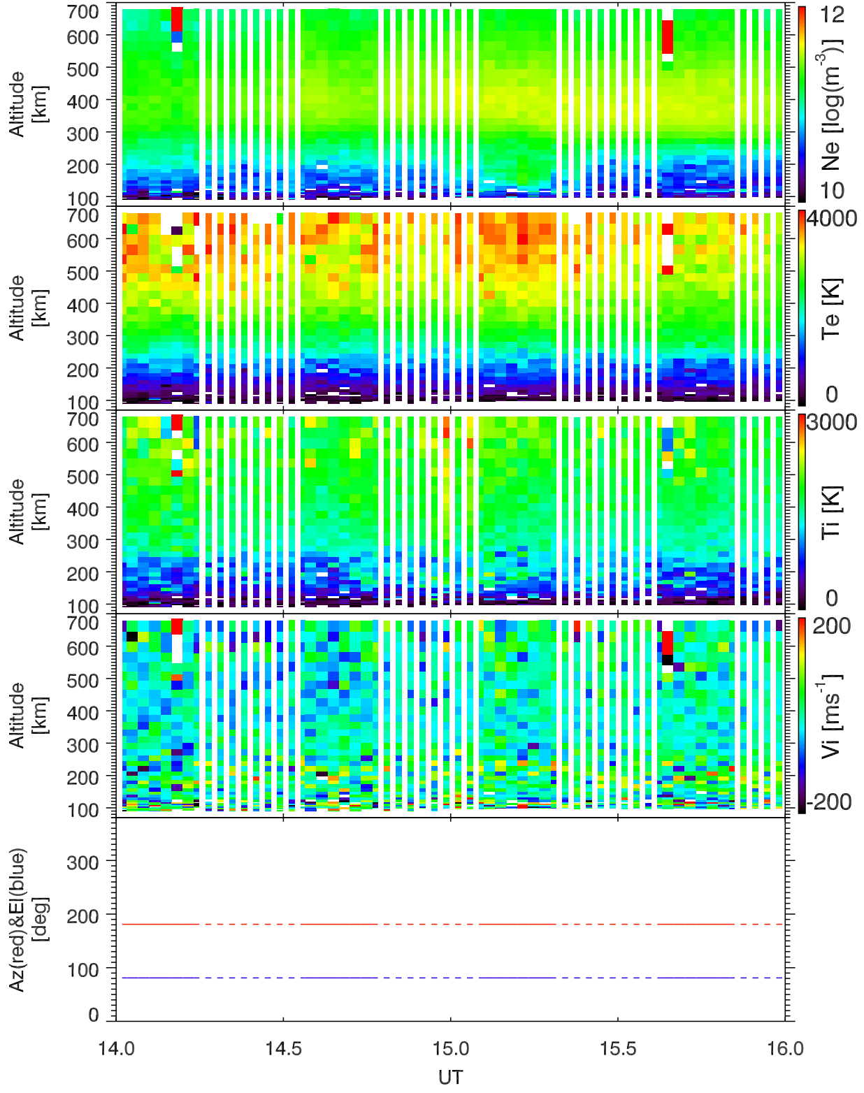
EISCAT 2001-10-01_14_16UT_tau0_120@42m.
