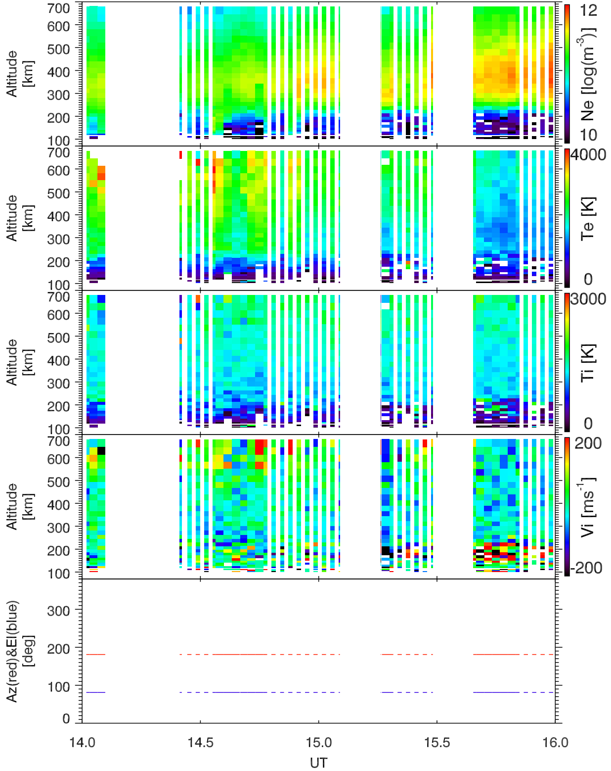
EISCAT 2001-10-30_14_16UT_tau0_120@42m.
