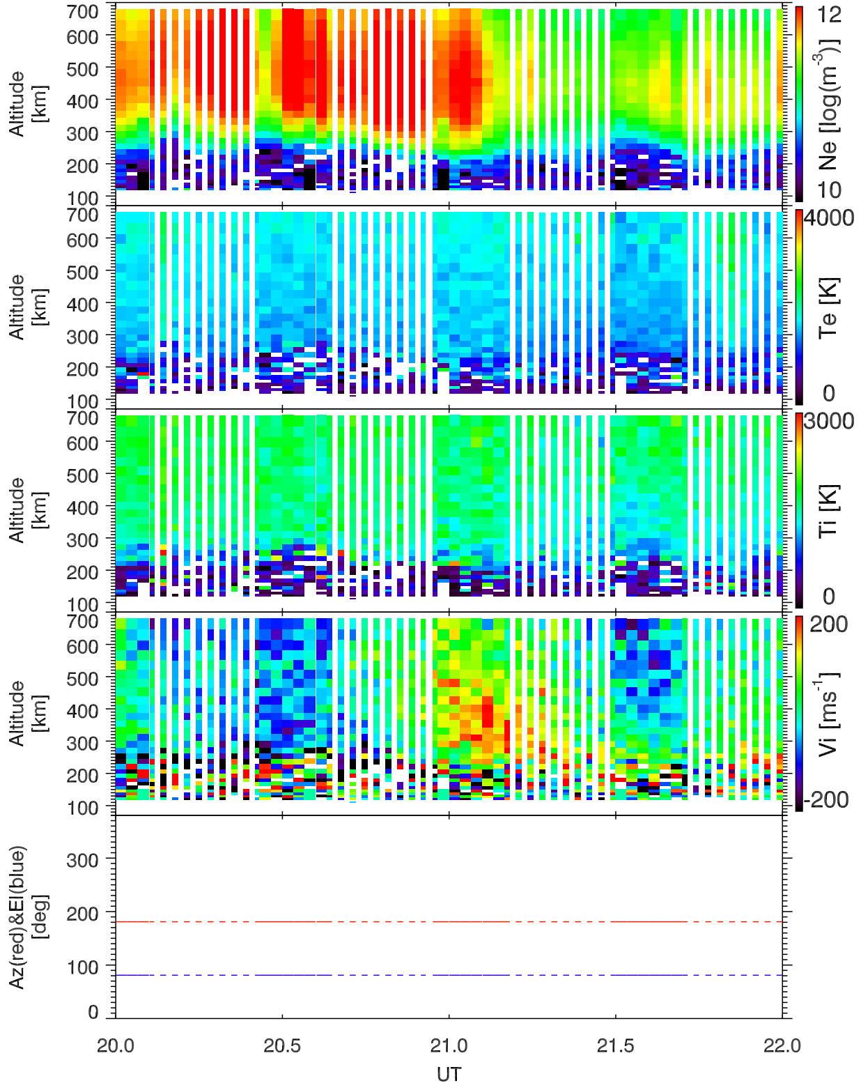
EISCAT 2001-11-05_20_22UT_tau0_120@42m.
