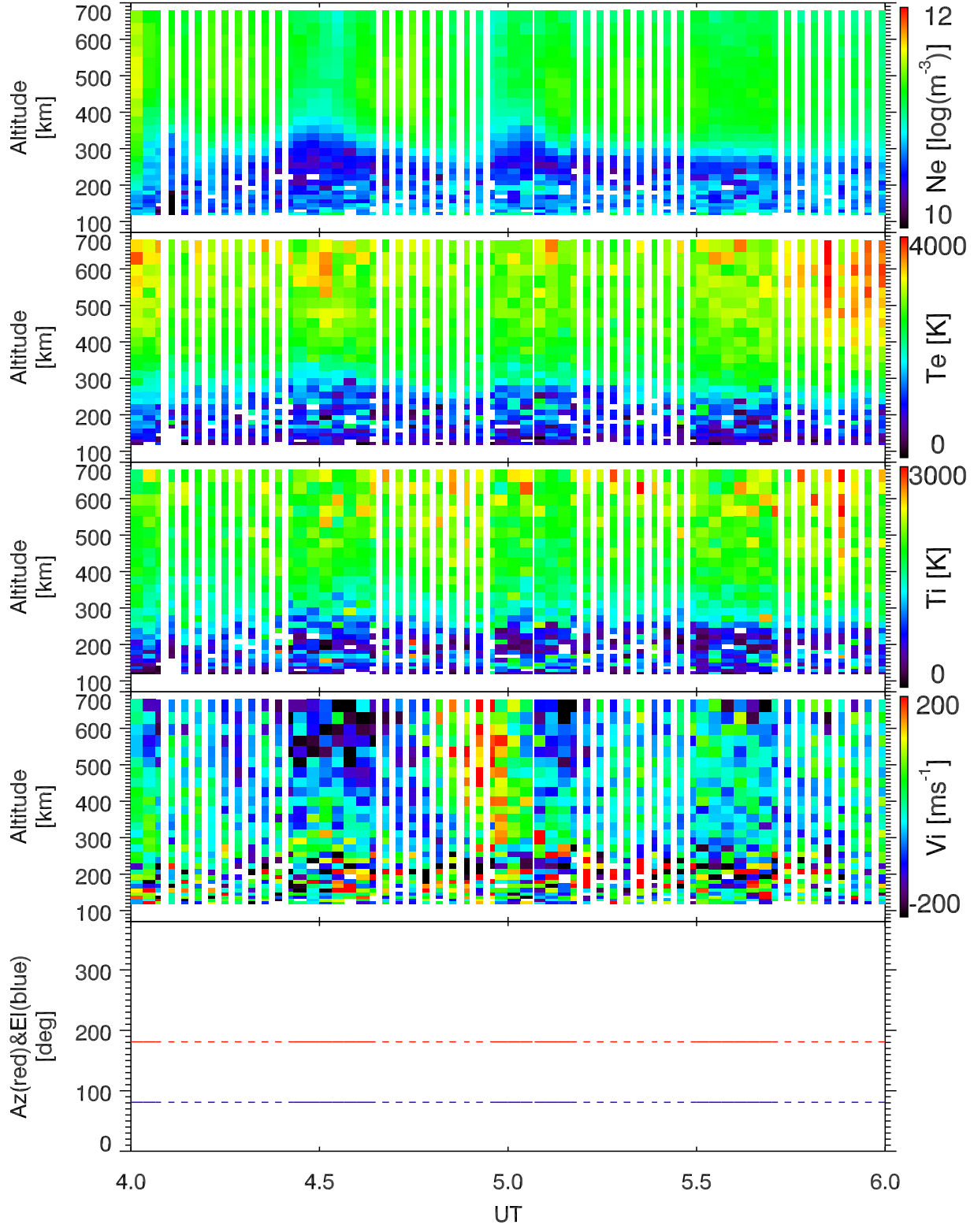
EISCAT 2001-11-06_04_06UT_tau0_120@42m.
