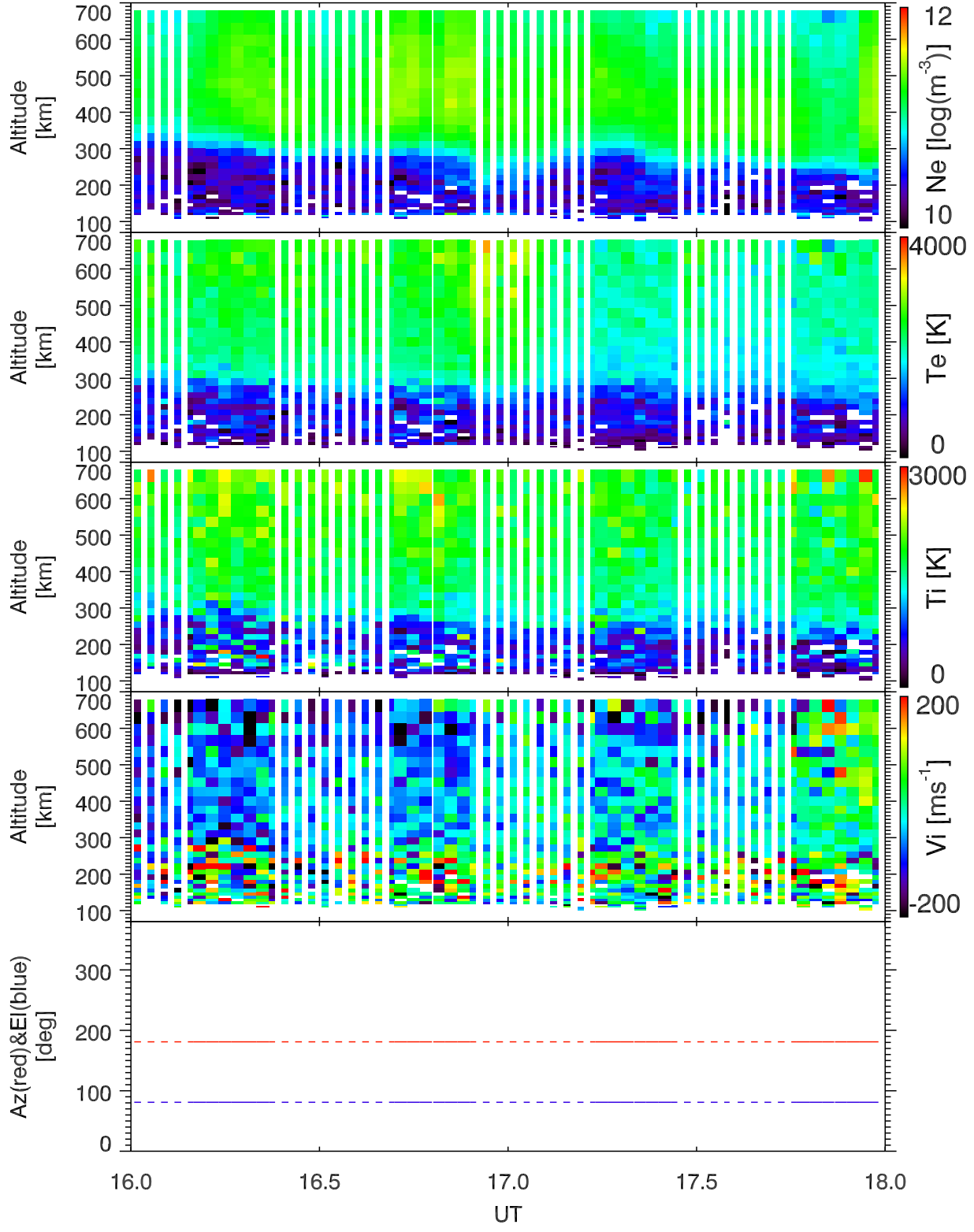
EISCAT 2001-11-06_16_18UT_tau0_120@42m.
