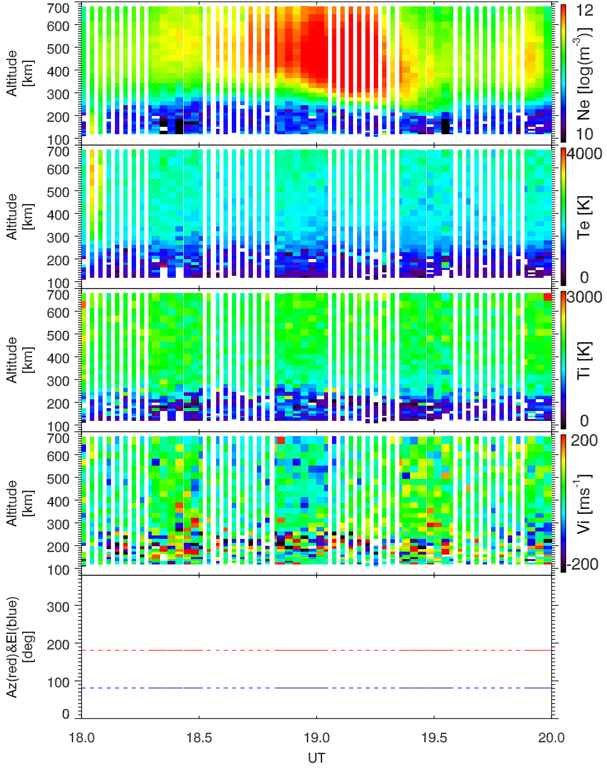
EISCAT 2001-11-06_18_20UT_tau0_120@42m.
