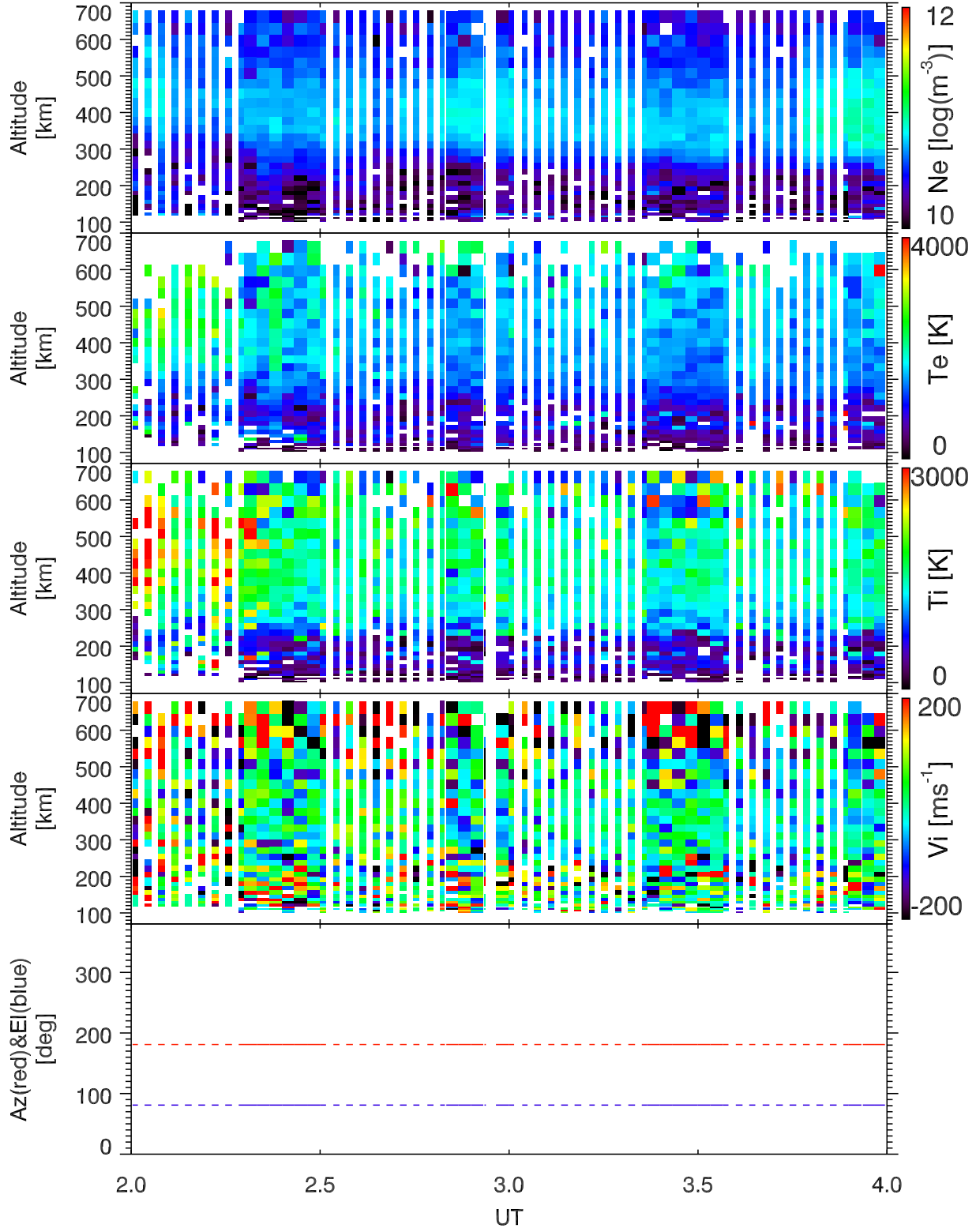
EISCAT 2001-11-07_02_04UT_tau0_120@42m.
