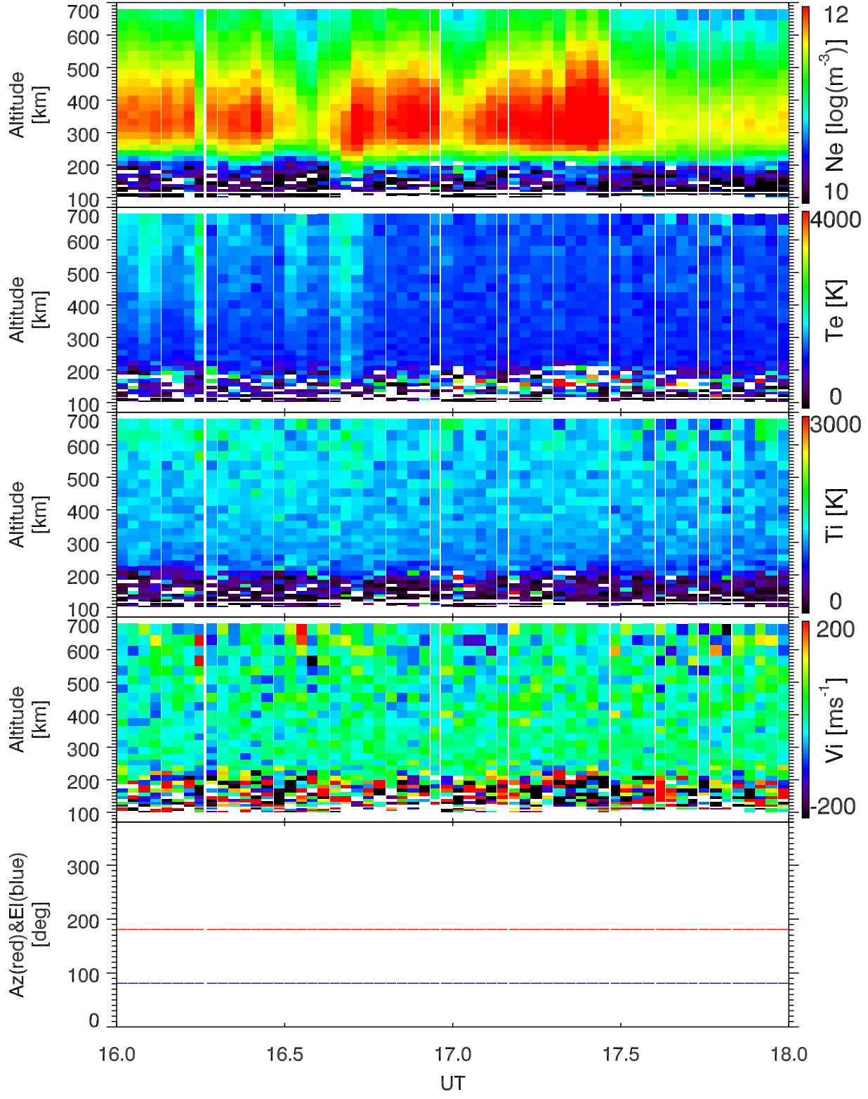
EISCAT 2001-11-13_16_18UT_tau0_120@42m.
