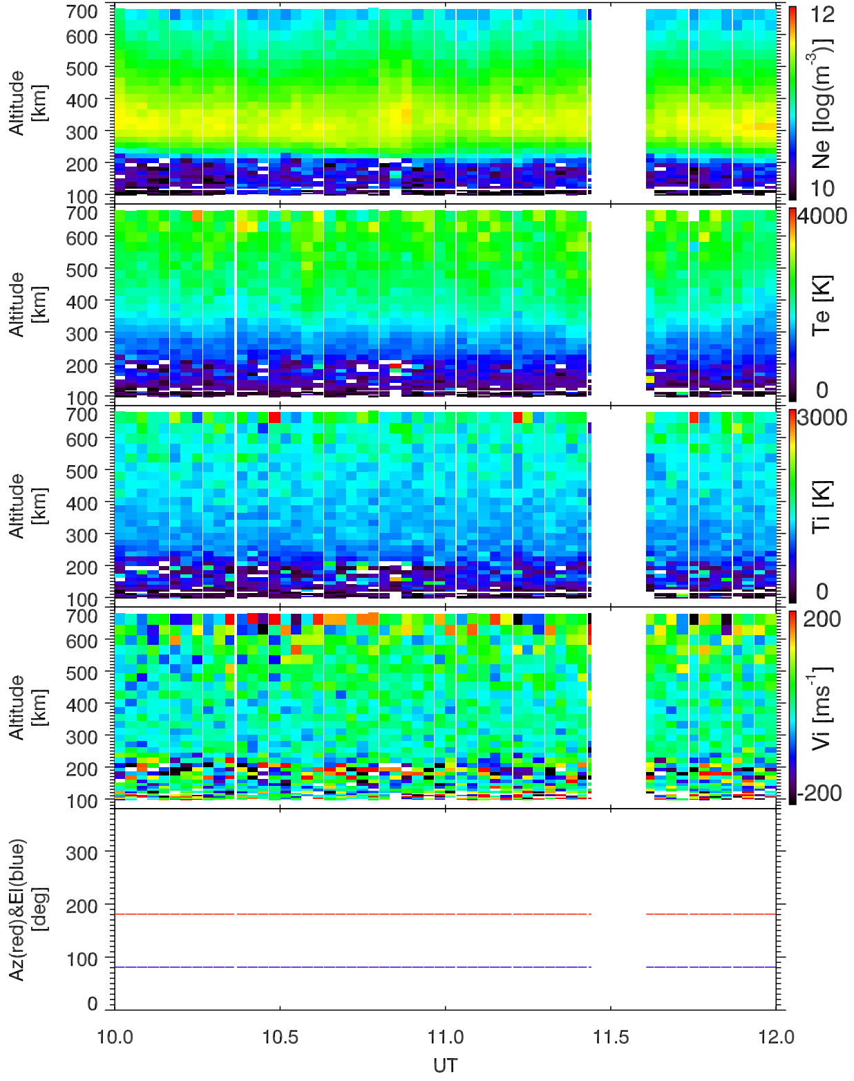
EISCAT 2001-11-14_10_12UT_tau0_120@42m.
