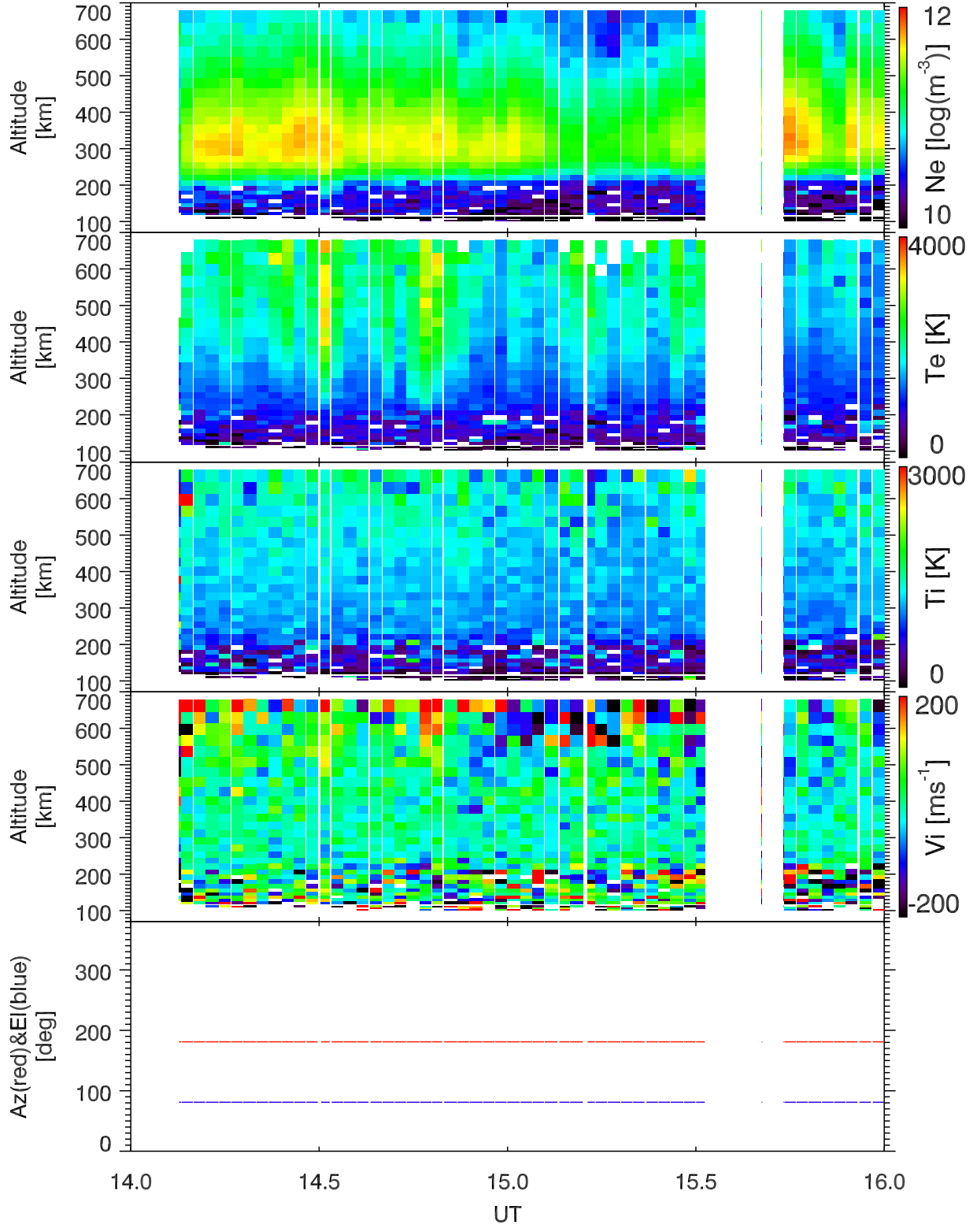
EISCAT 2001-11-14_14_16UT_tau0_120@42m.
