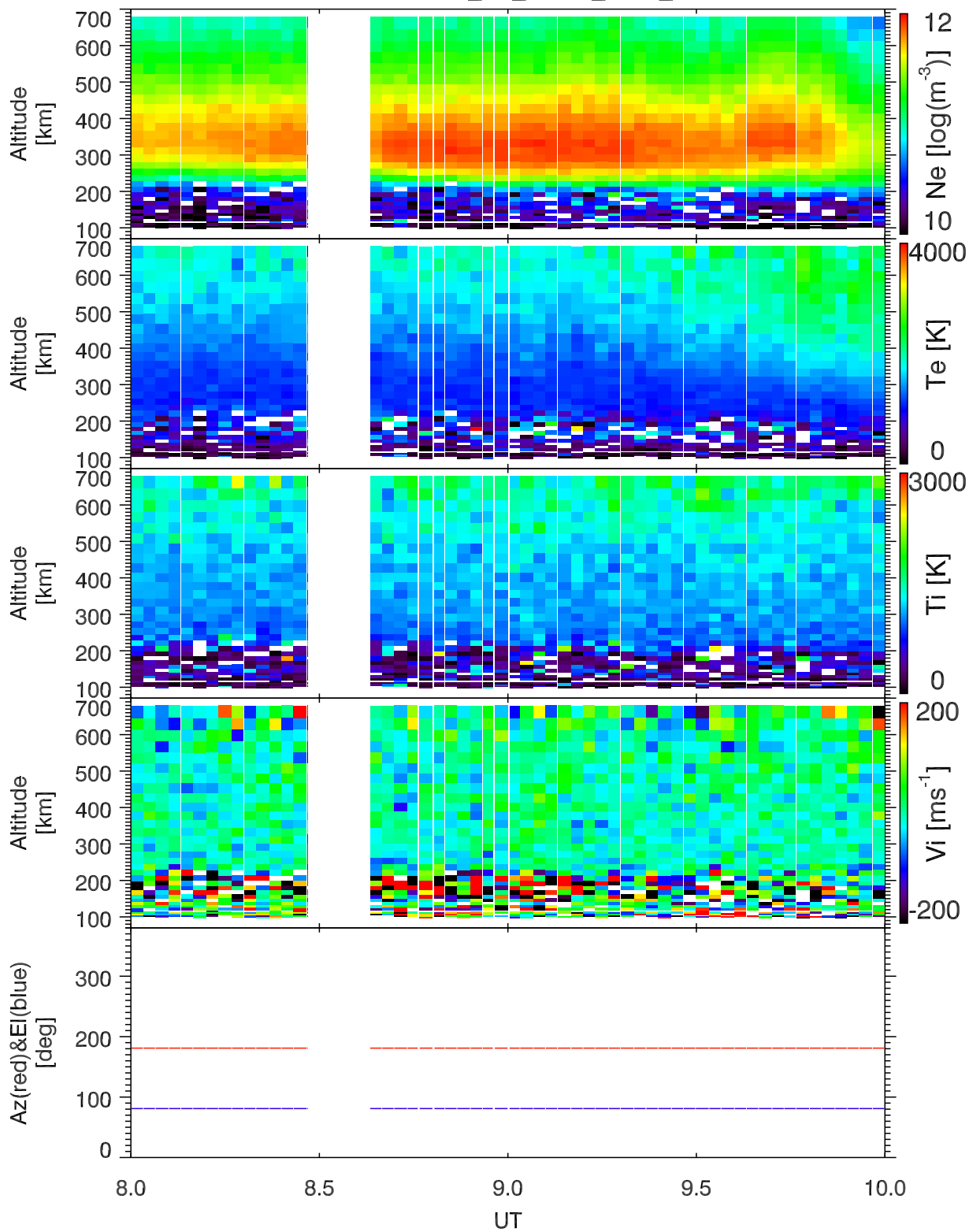
EISCAT 2001-11-15_08_10UT_tau0_all@42m.
