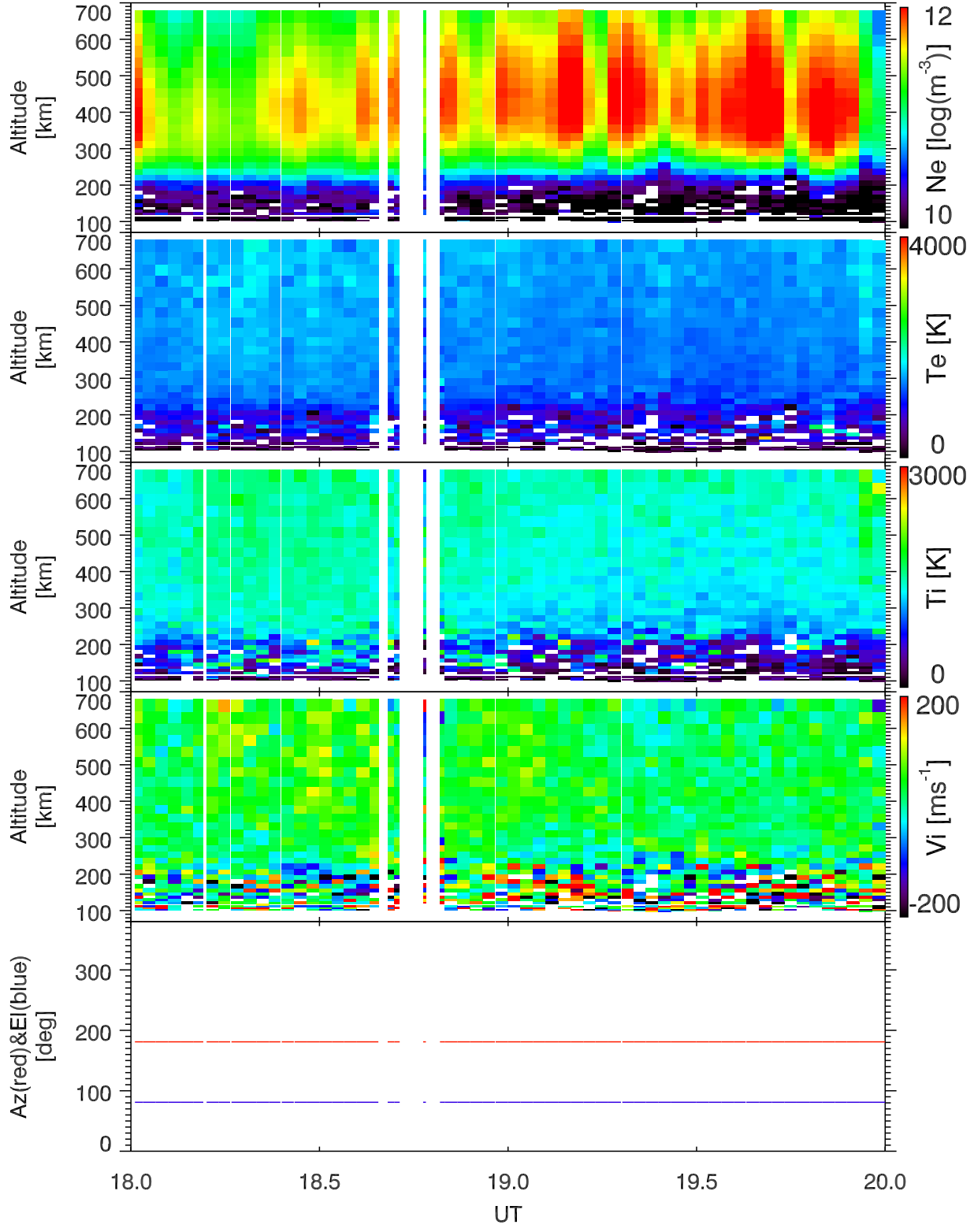
EISCAT 2001-11-17_18_20UT_tau0_120@42m.
