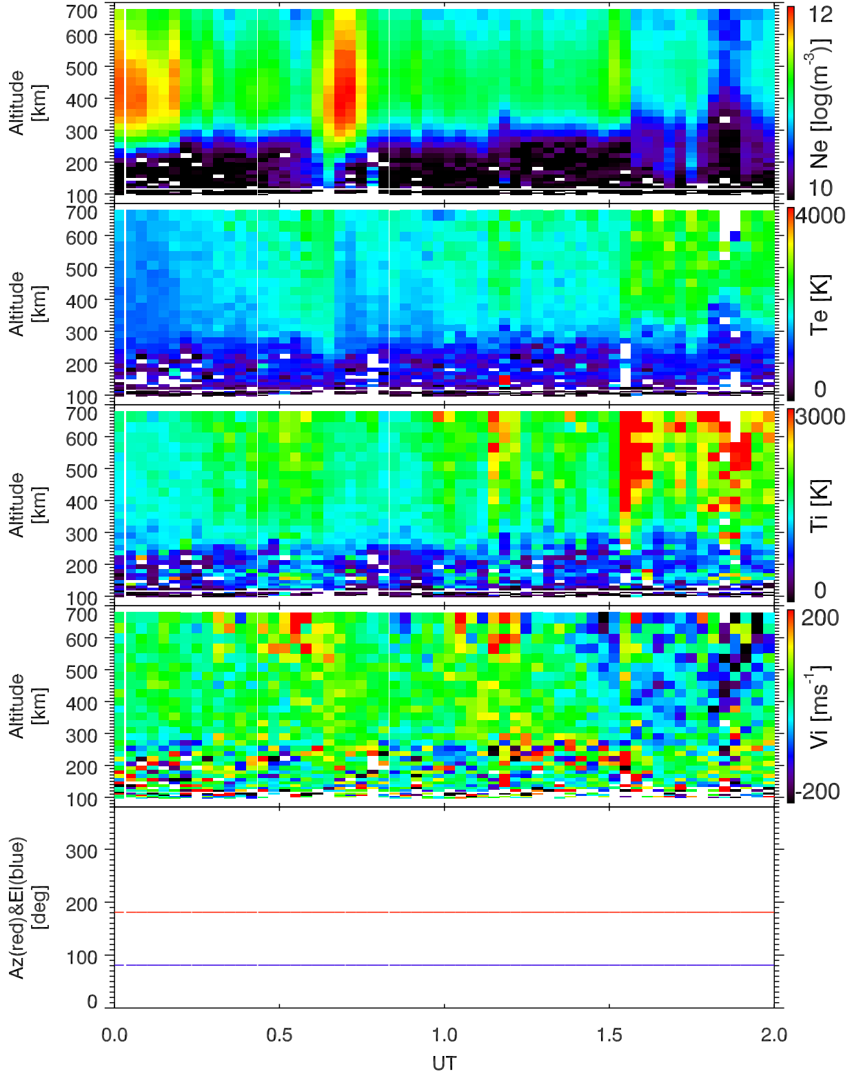
EISCAT 2001-11-18_00_02UT_tau0_all@42m.
