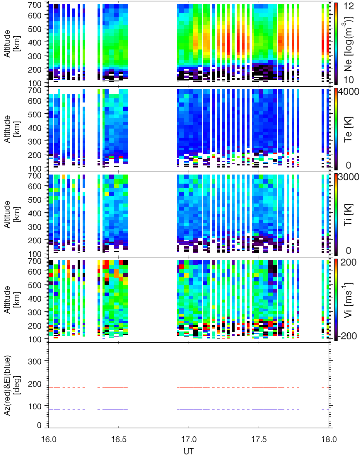
EISCAT 2001-11-27_16_18UT_tau0_120@42m.
