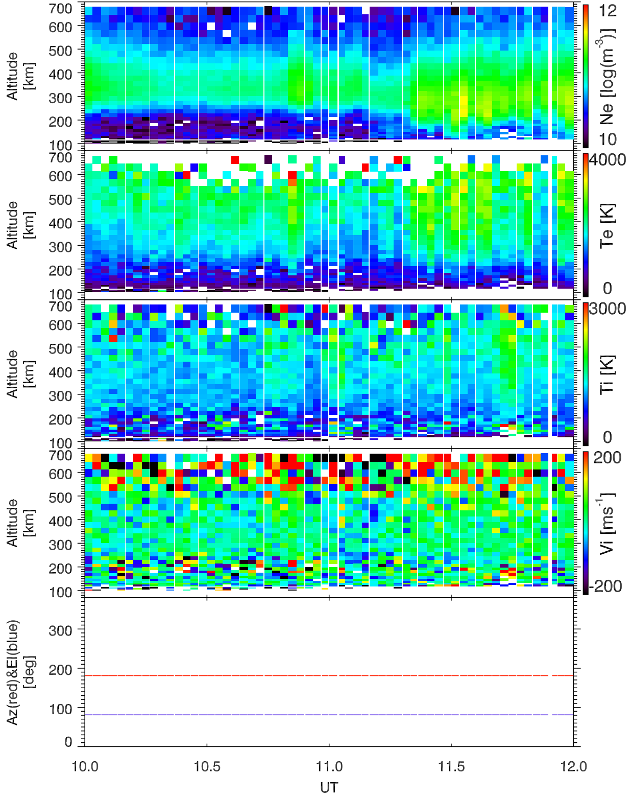
EISCAT 2001-12-11_10_12UT_tau0_120@42m.
