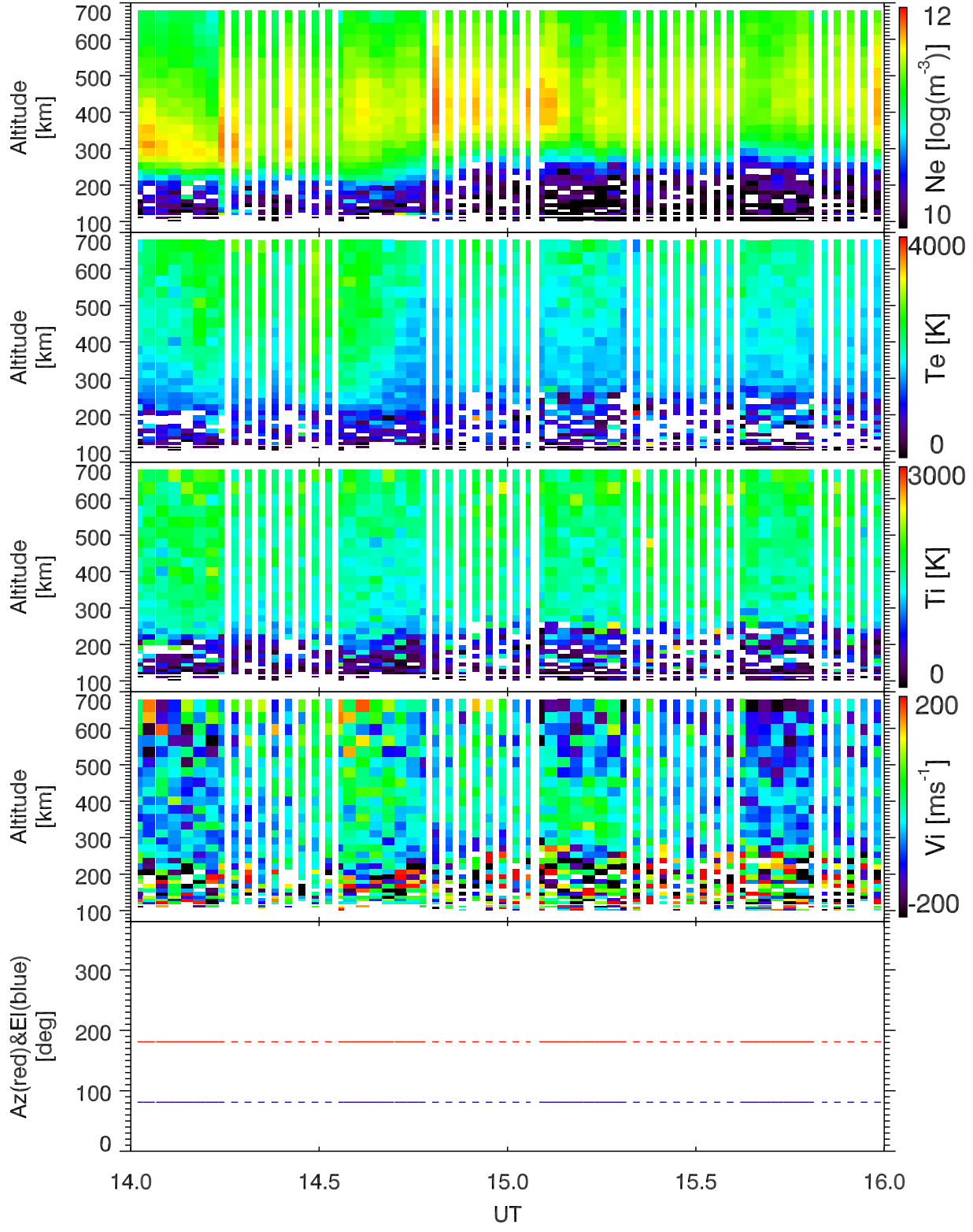
EISCAT 2001-12-12_14_16UT_tau0_120@42m.
