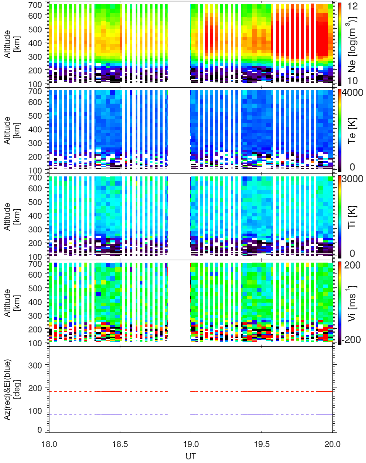
EISCAT 2001-12-12_18_20UT_tau0_120@42m.
