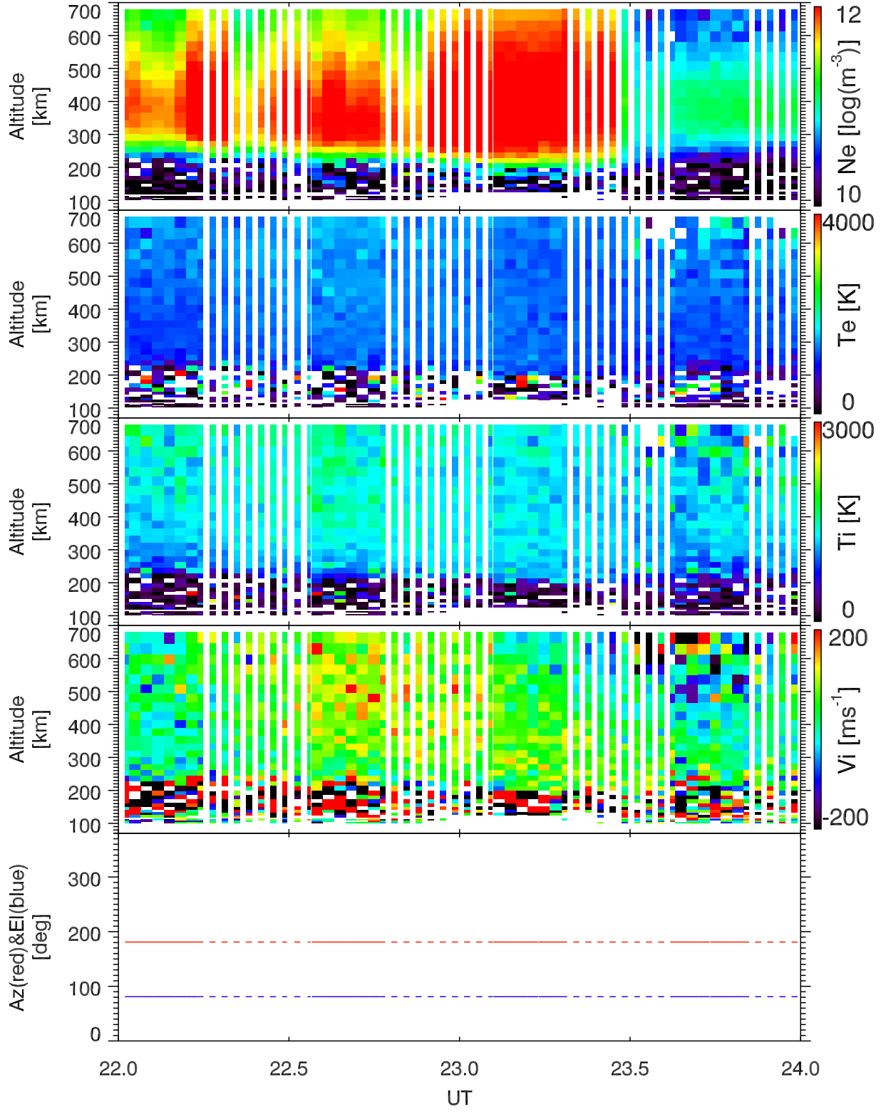
EISCAT 2001-12-12_22_24UT_tau0_120@42m.
