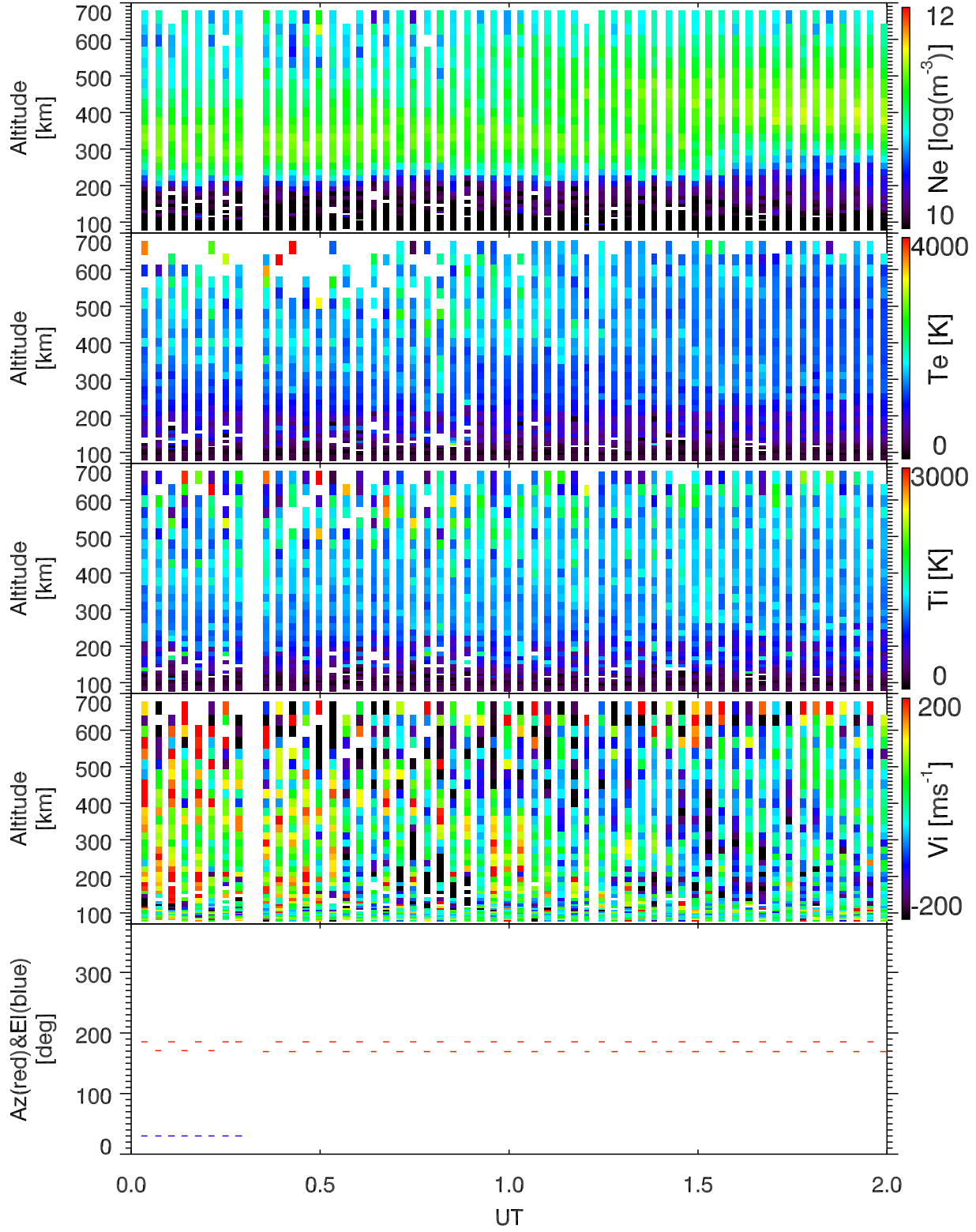
EISCAT 2001-12-14_00_02UT_tau0_ant@32m.
