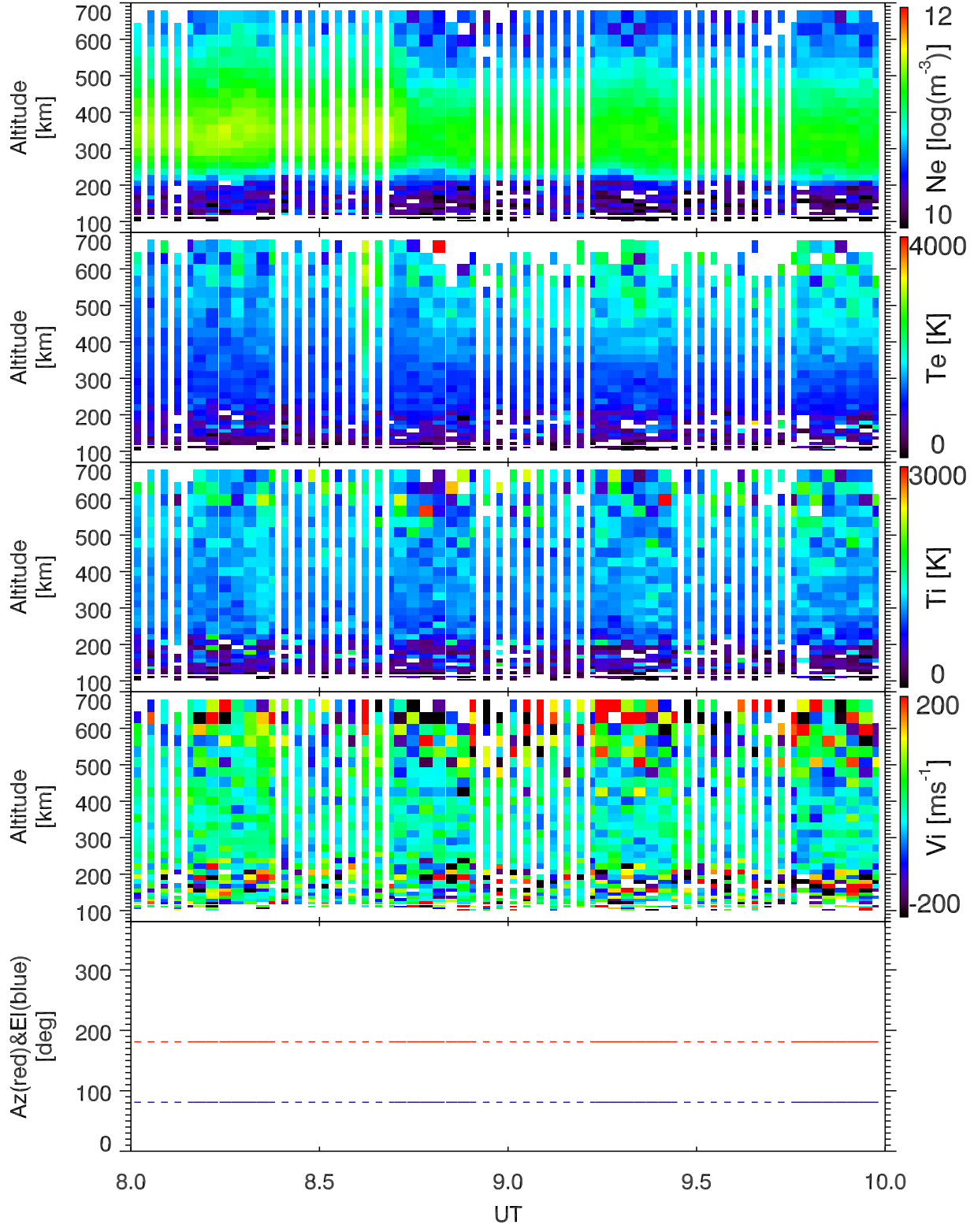
EISCAT 2001-12-14_08_10UT_tau0_120@42m.
