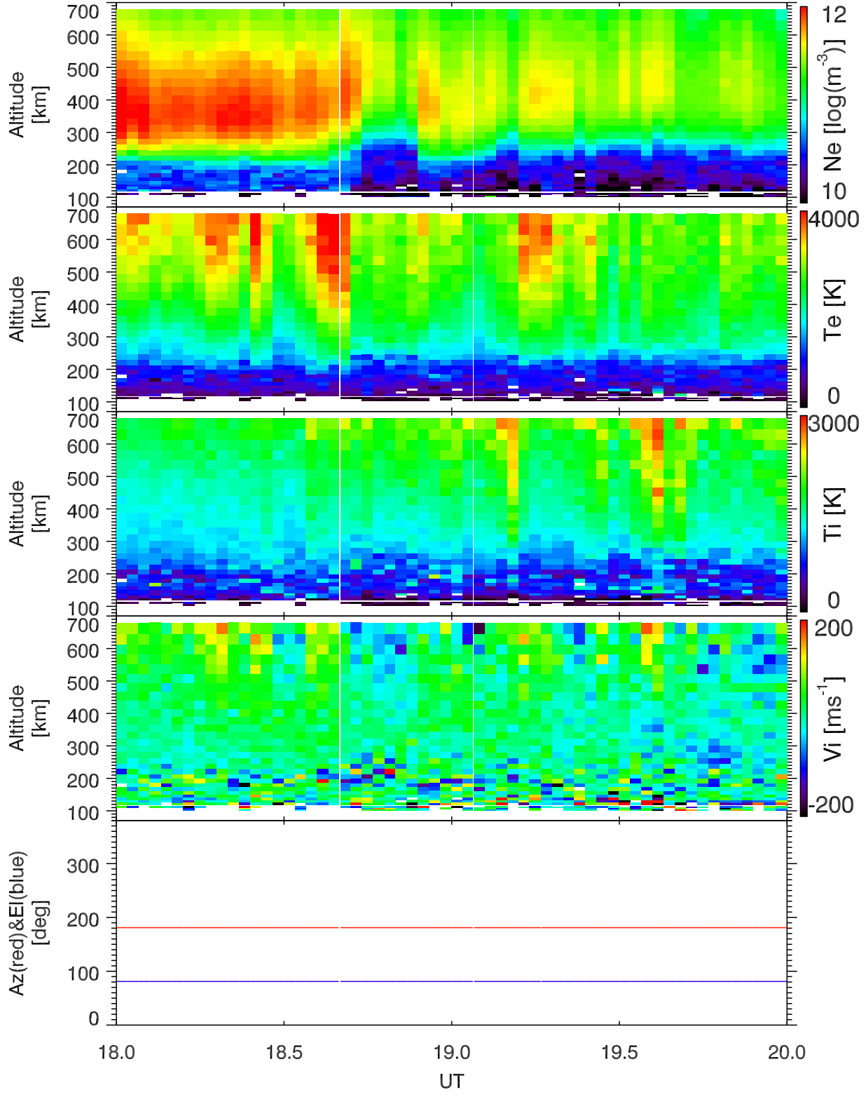
EISCAT 2001-12-15_18_20UT_tau0_120@42m.
