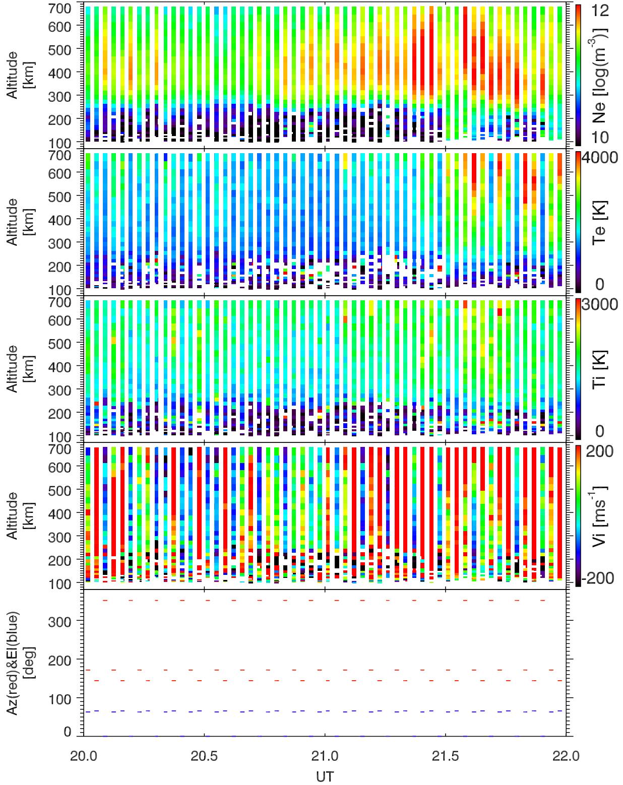
EISCAT 2002-01-20_20_22UT_tau0_all@32m.
