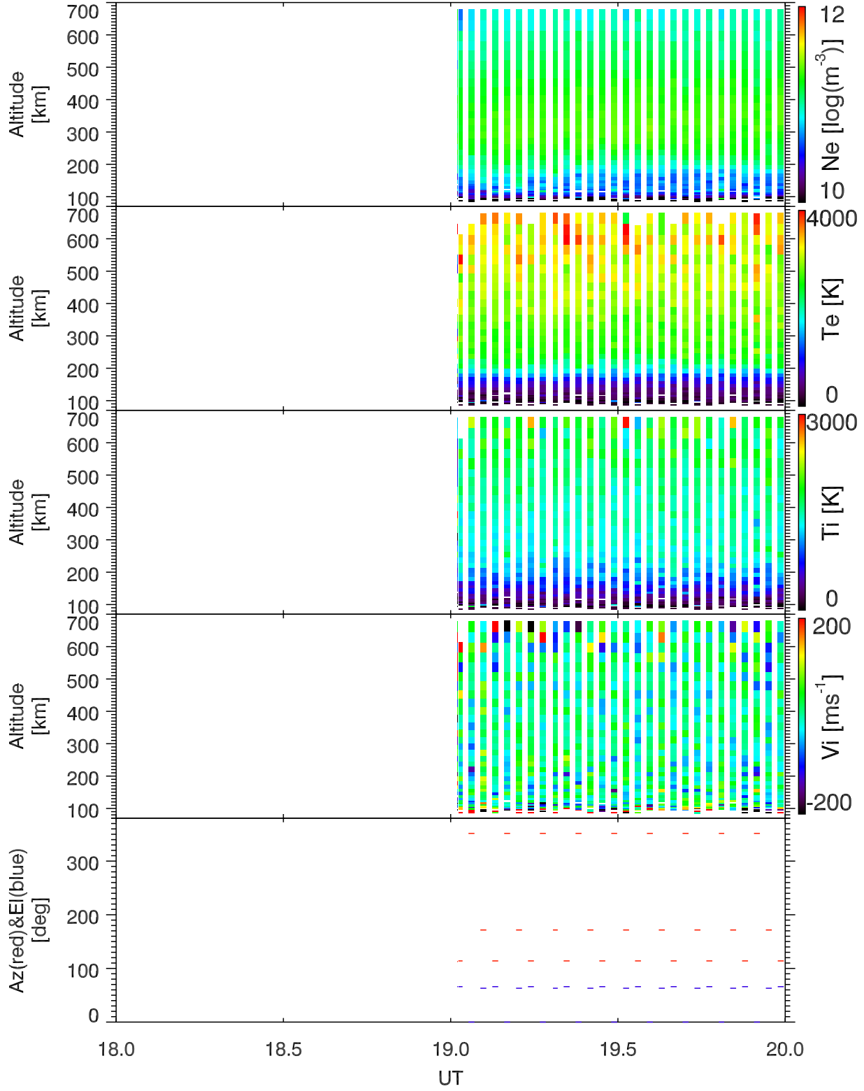
EISCAT 2002-07-31_18_20UT_tau0_ant@32m.
