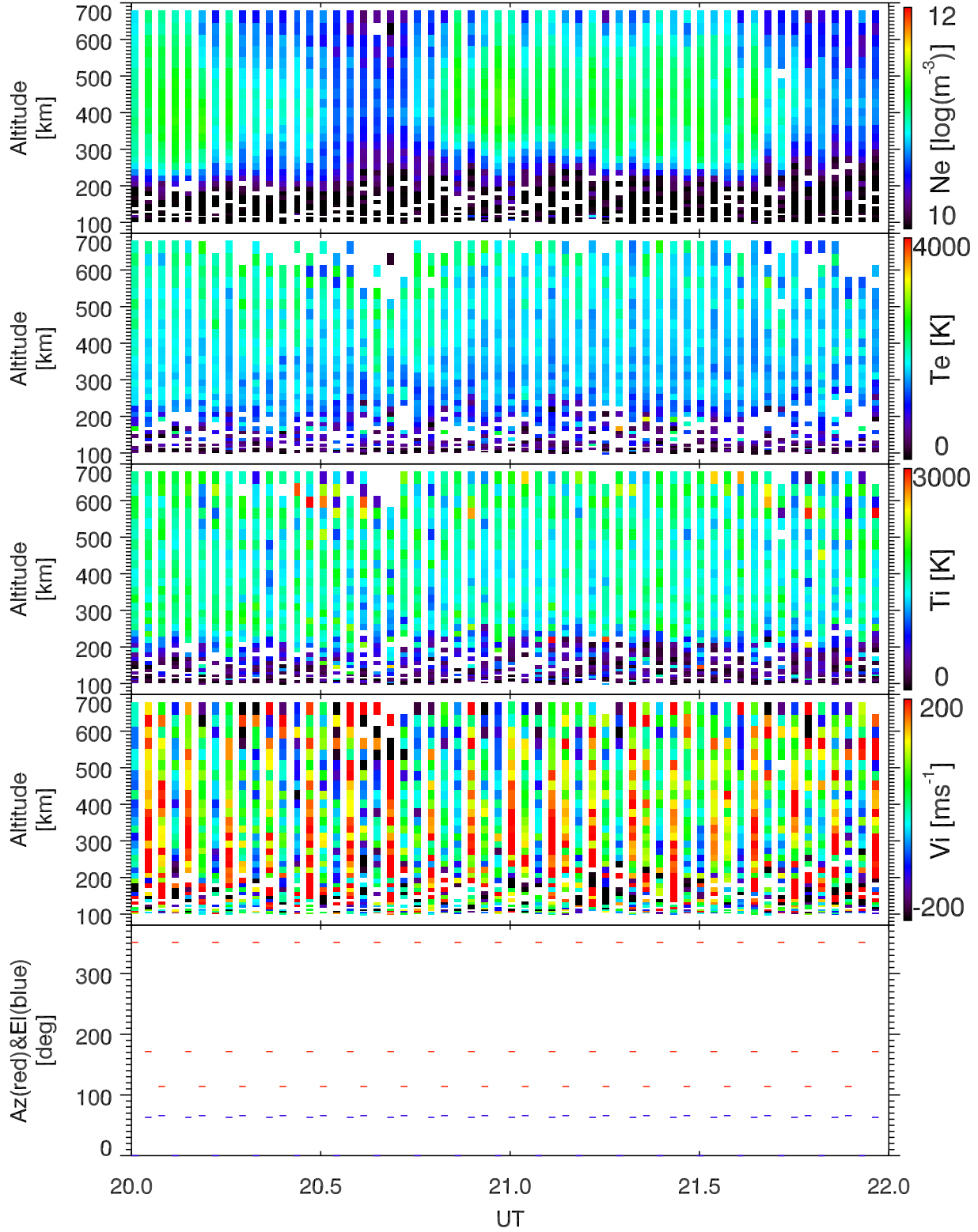
EISCAT 2002-10-04_20_22UT_tau0_ant@32m.
