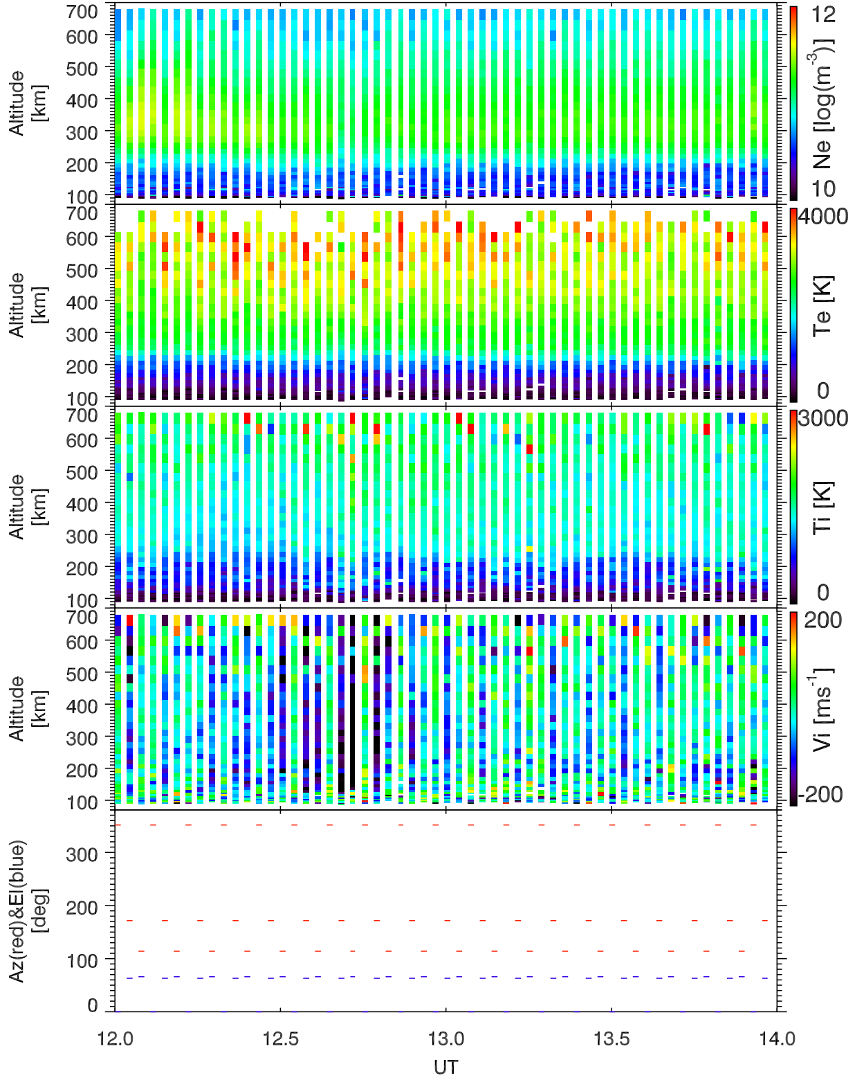
EISCAT 2002-10-05_12_14UT_tau0_ant@32m.
