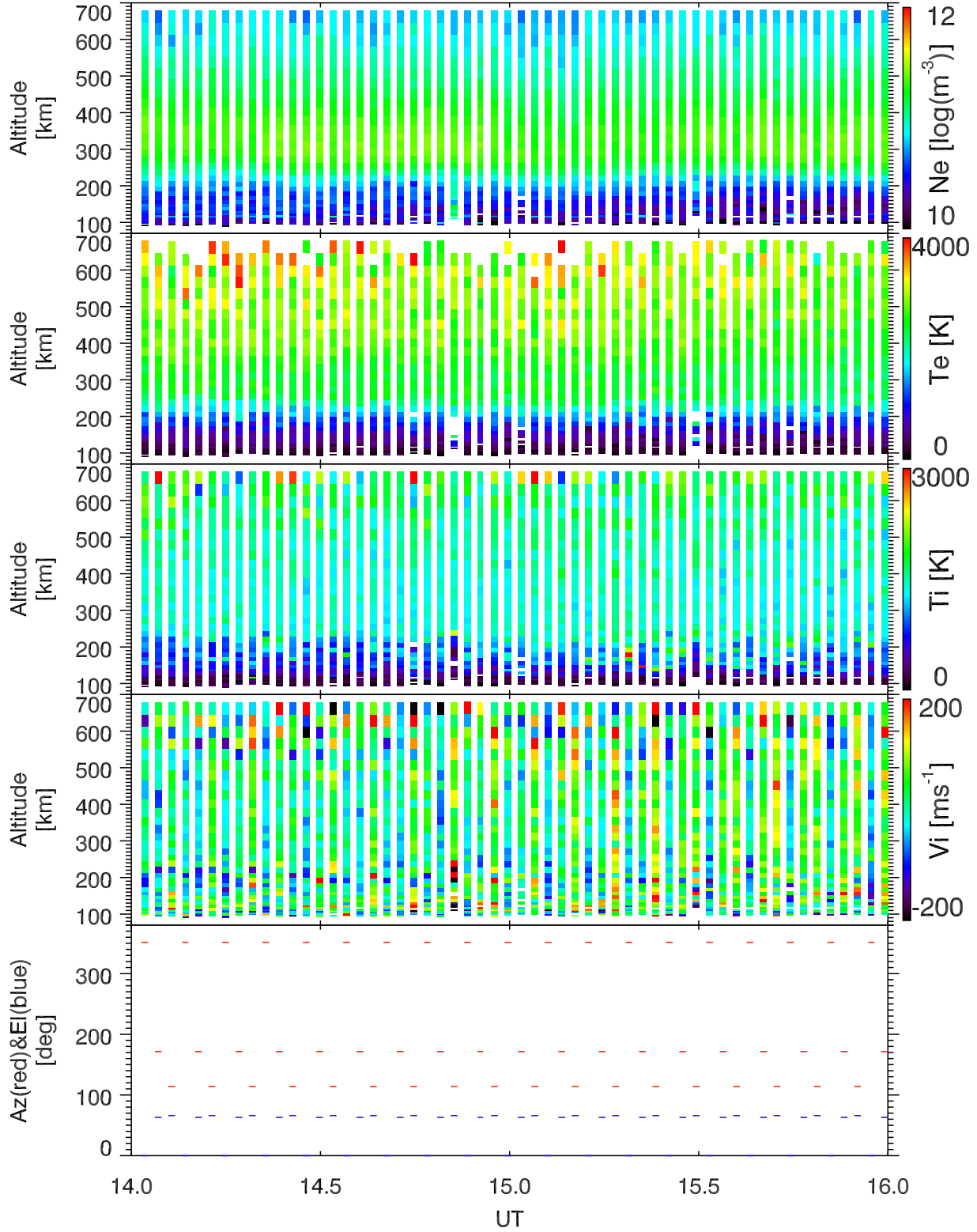
EISCAT 2002-10-05_14_16UT_tau0_ant@32m.
