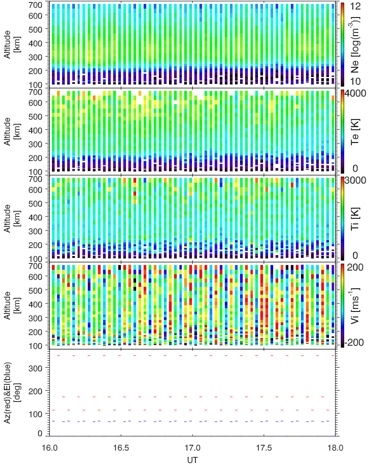
EISCAT 2002-10-05_16_18UT_tau0_ant@32m.
