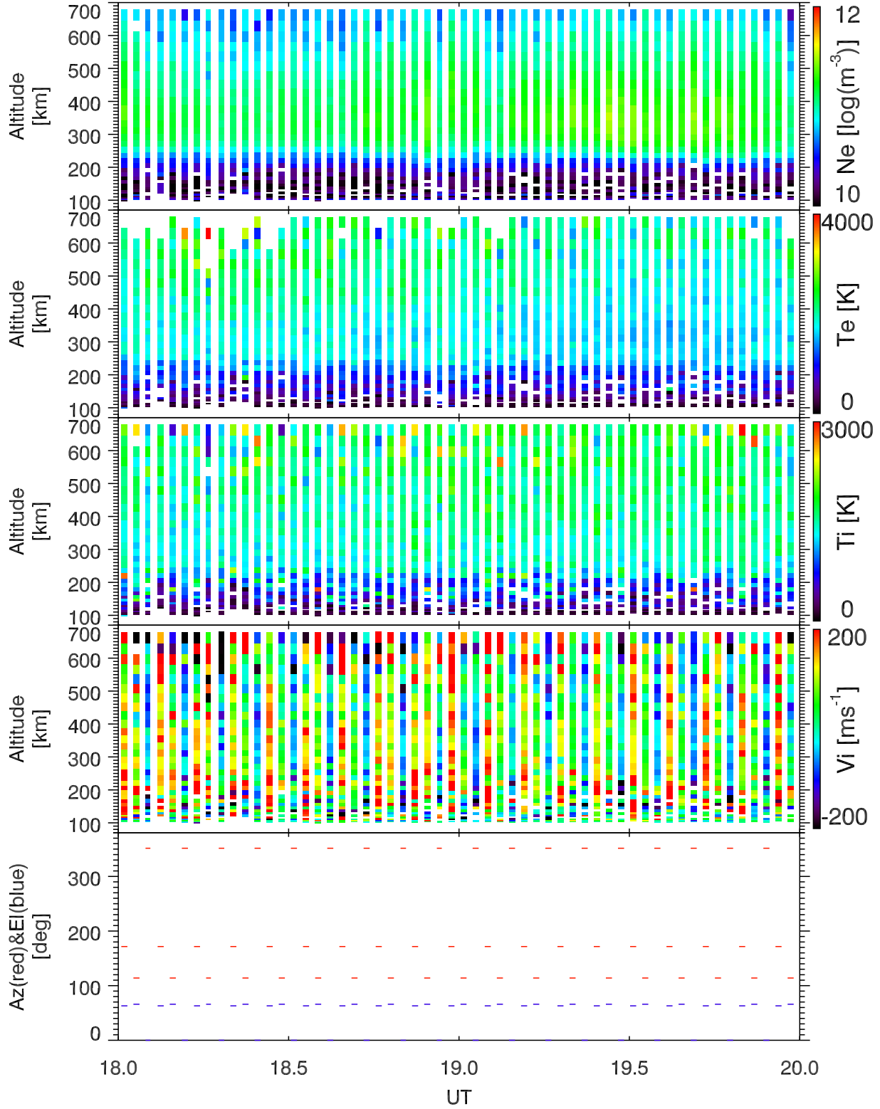
EISCAT 2002-10-05_18_20UT_tau0_ant@32m.
