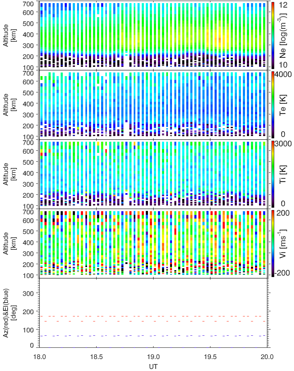
EISCAT 2002-10-06_18_20UT_tau0_ant@32m.
