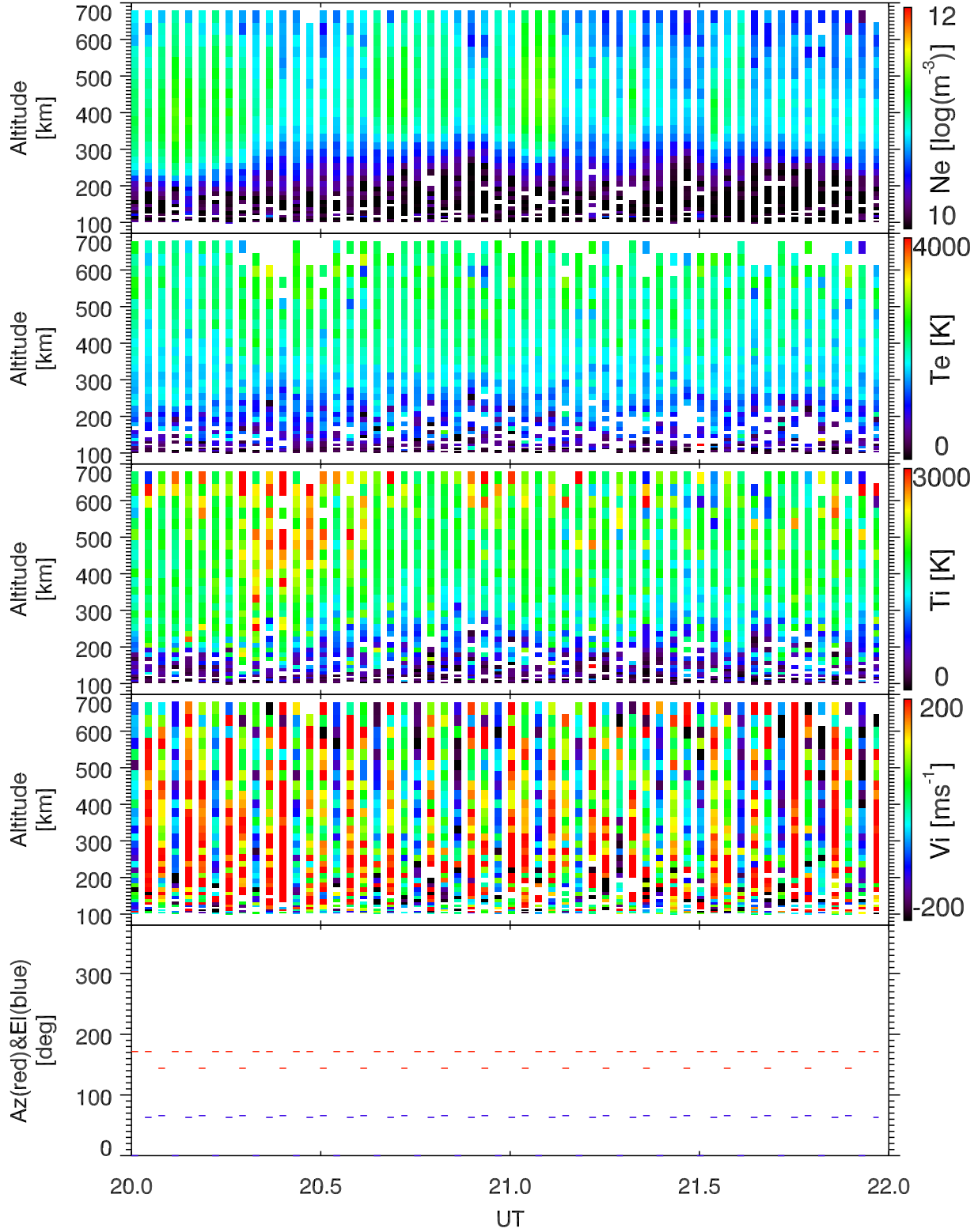
EISCAT 2002-10-07_20_22UT_tau0_ant@32m.
