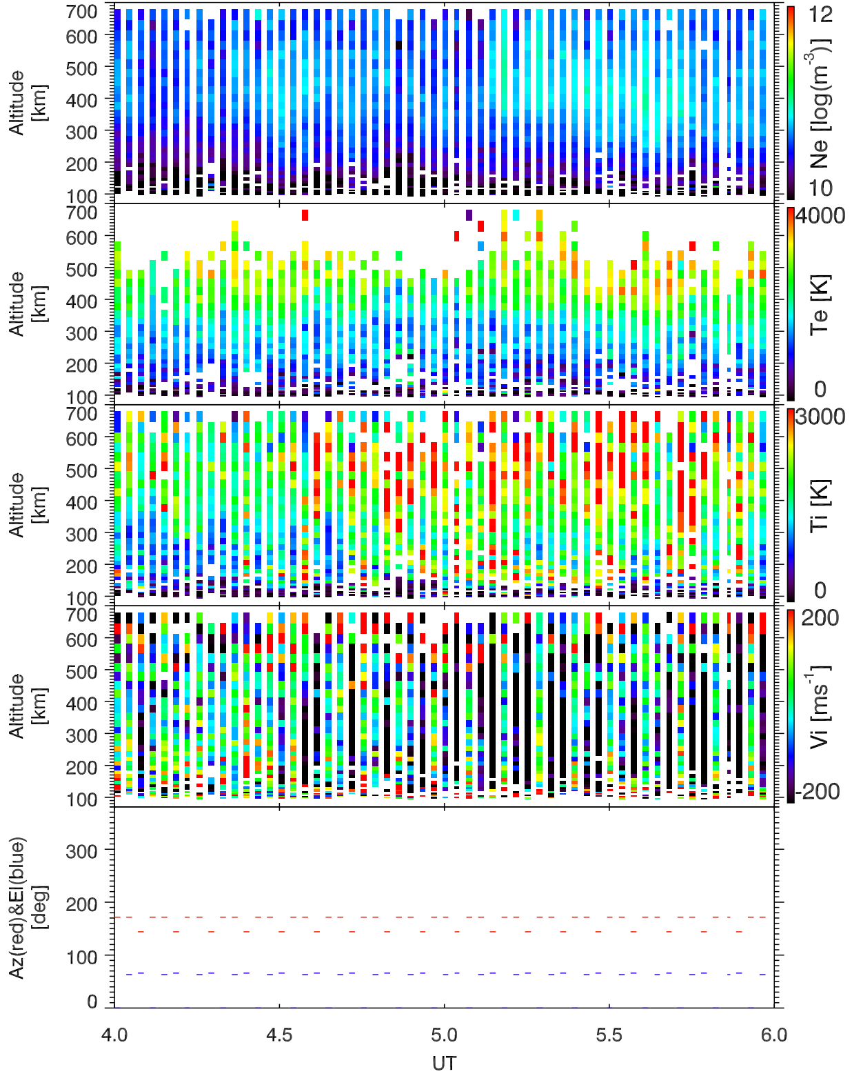
EISCAT 2002-10-08_04_06UT_tau0_ant@32m.
