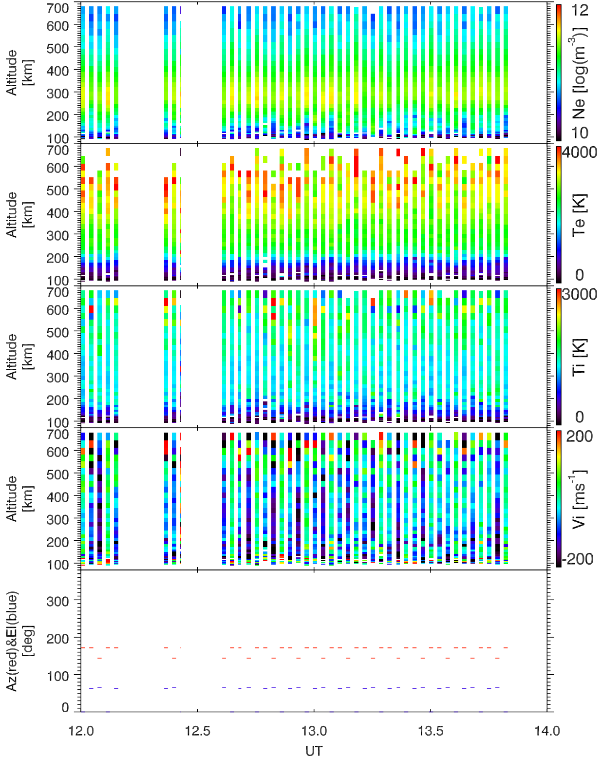
EISCAT 2002-10-11_12_14UT_tau0_ant@32m.
