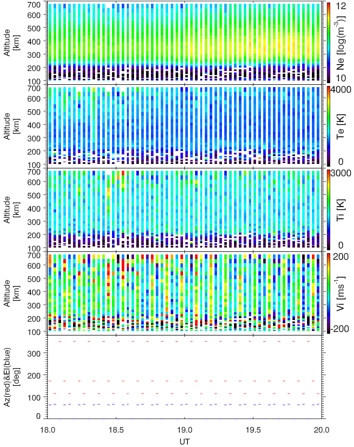
EISCAT 2002-10-11_18_20UT_tau0_ant@32m.
