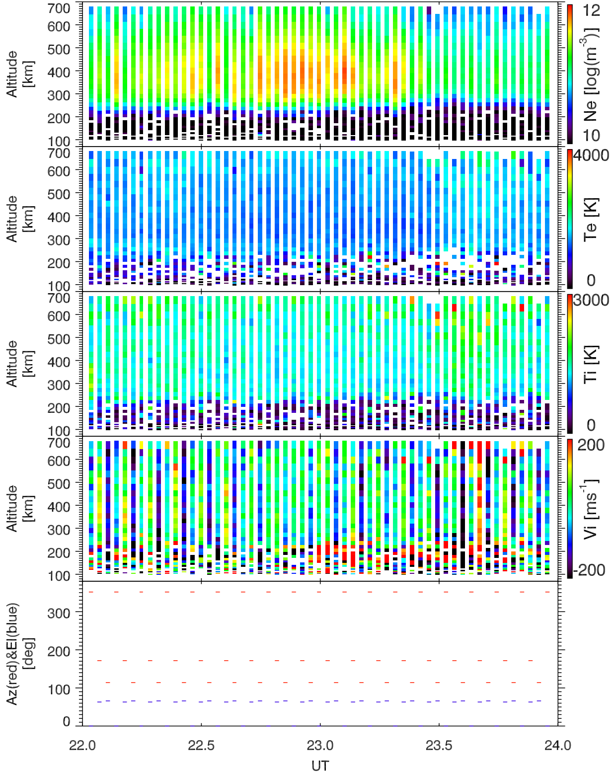
EISCAT 2002-10-11_22_24UT_tau0_ant@32m.
