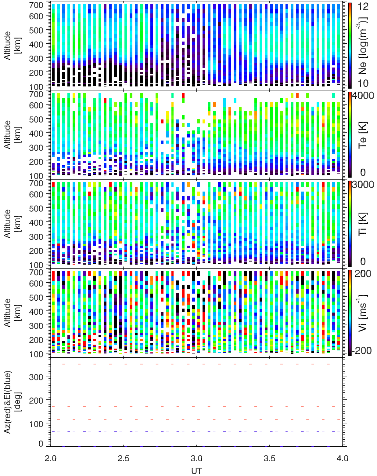
EISCAT 2002-10-13_02_04UT_tau0_ant@32m.
