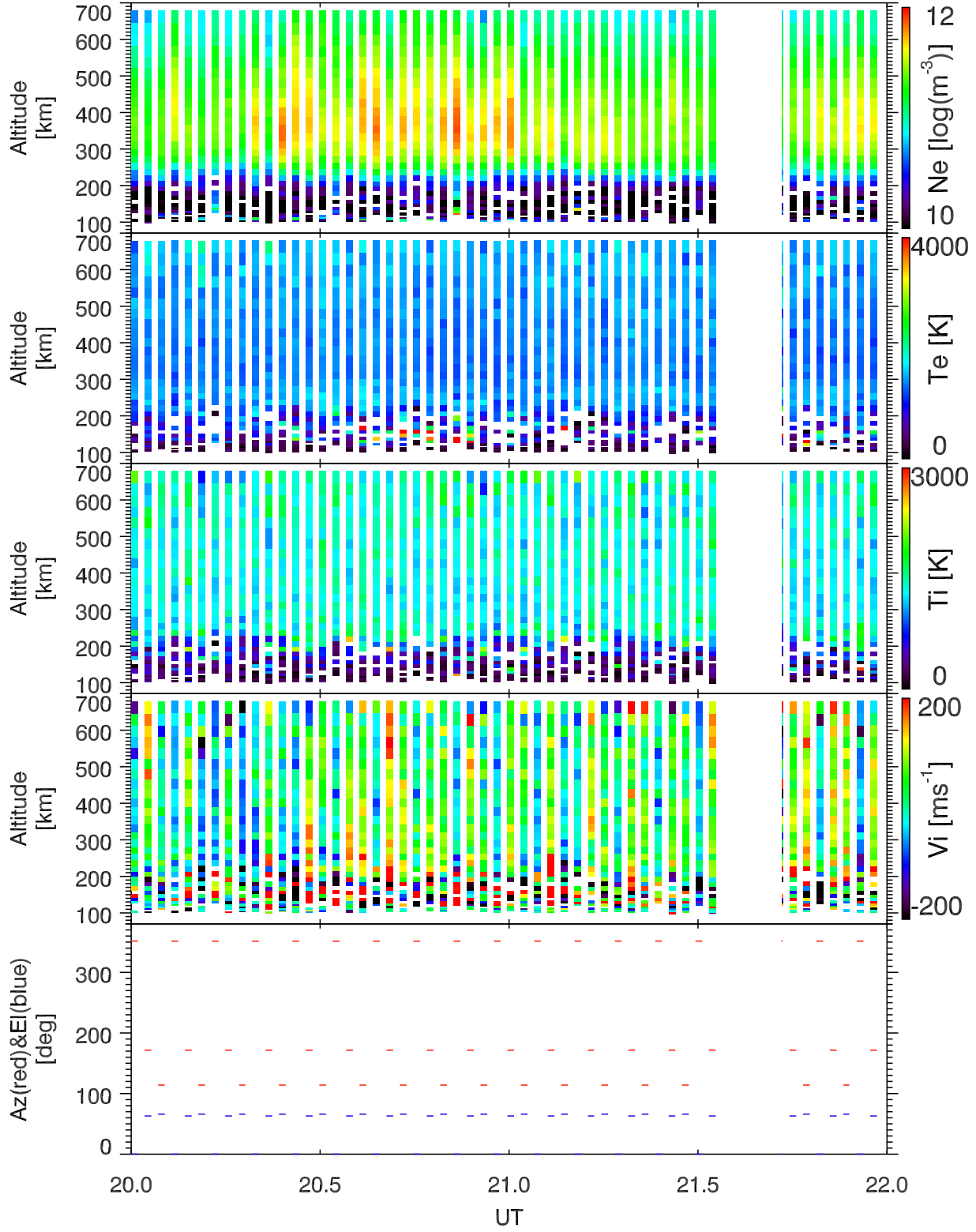
EISCAT 2002-10-13_20_22UT_tau0_ant@32m.
