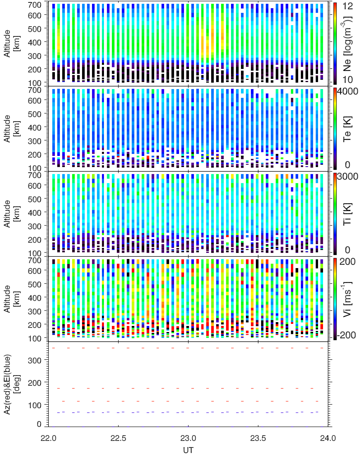
EISCAT 2002-10-13_22_24UT_tau0_ant@32m.
