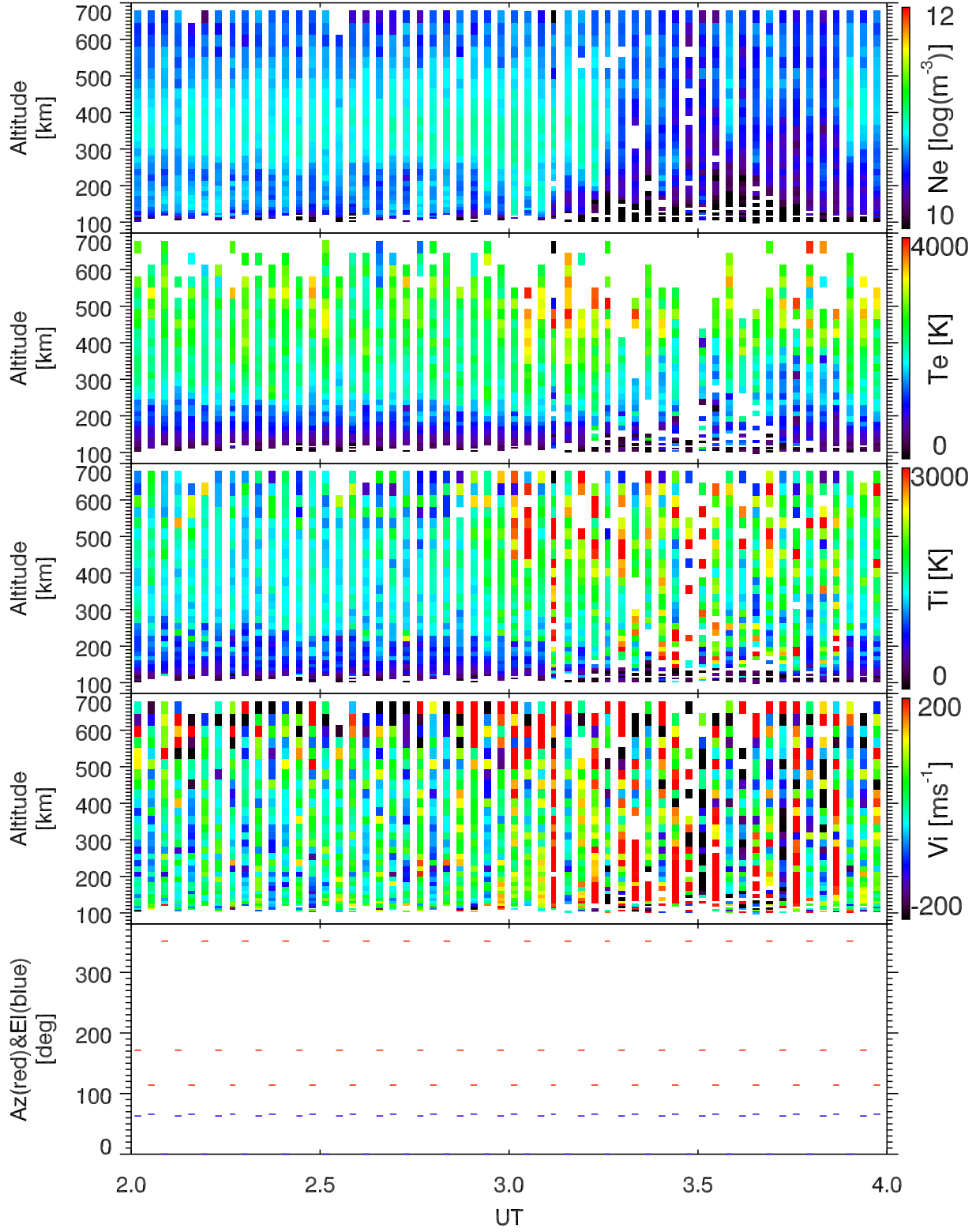
EISCAT 2002-10-15_02_04UT_tau0_ant@32m.
