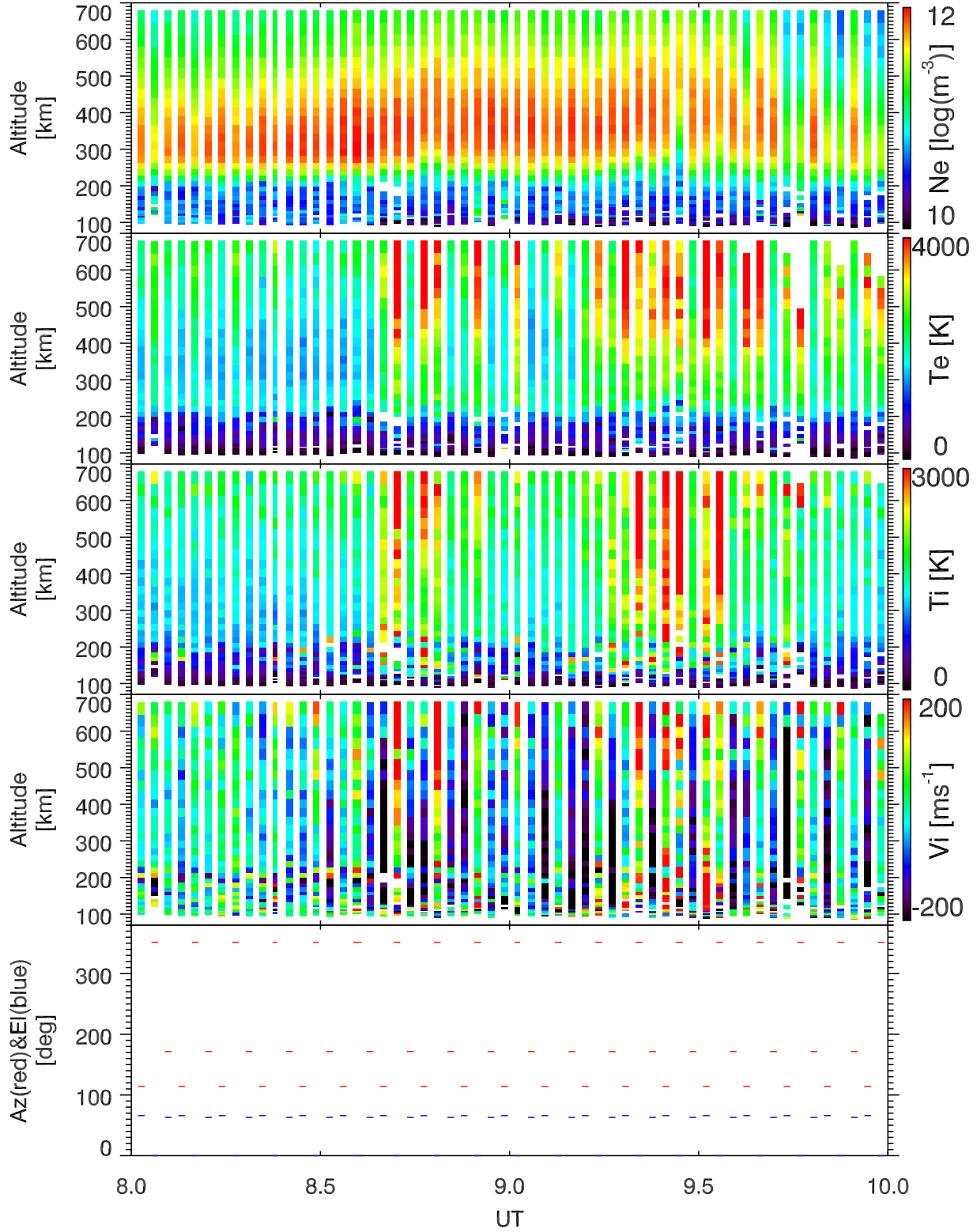
EISCAT 2002-10-15_08_10UT_tau0_ant@32m.
