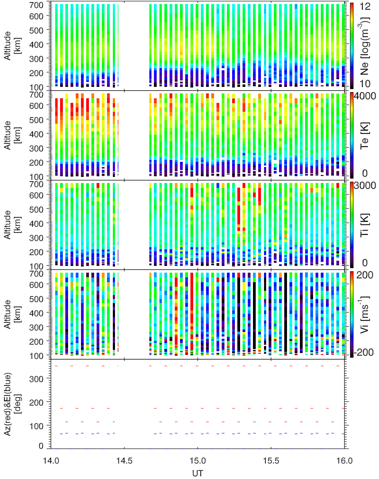
EISCAT 2002-10-15_14_16UT_tau0_ant@32m.
