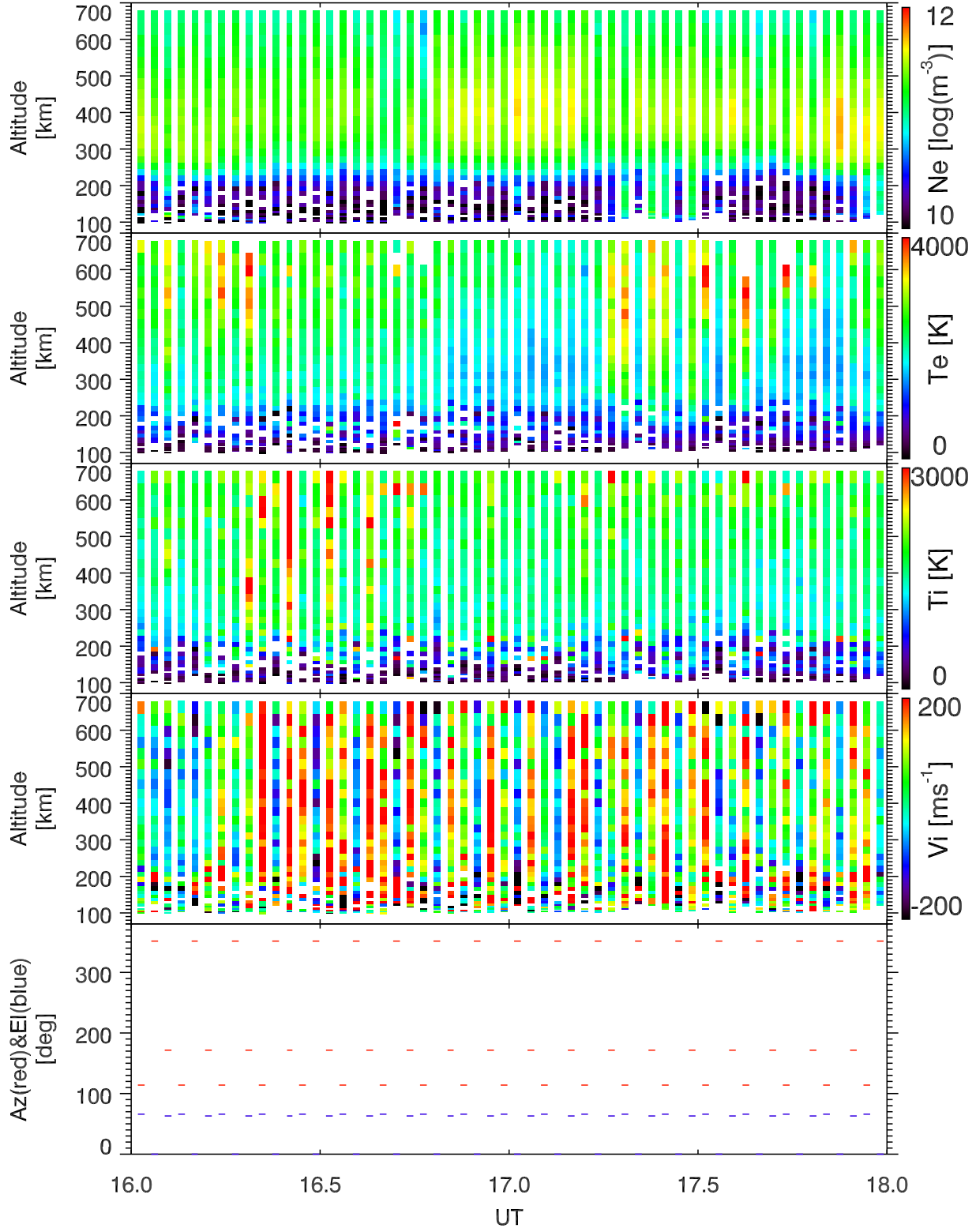
EISCAT 2002-10-15_16_18UT_tau0_ant@32m.
