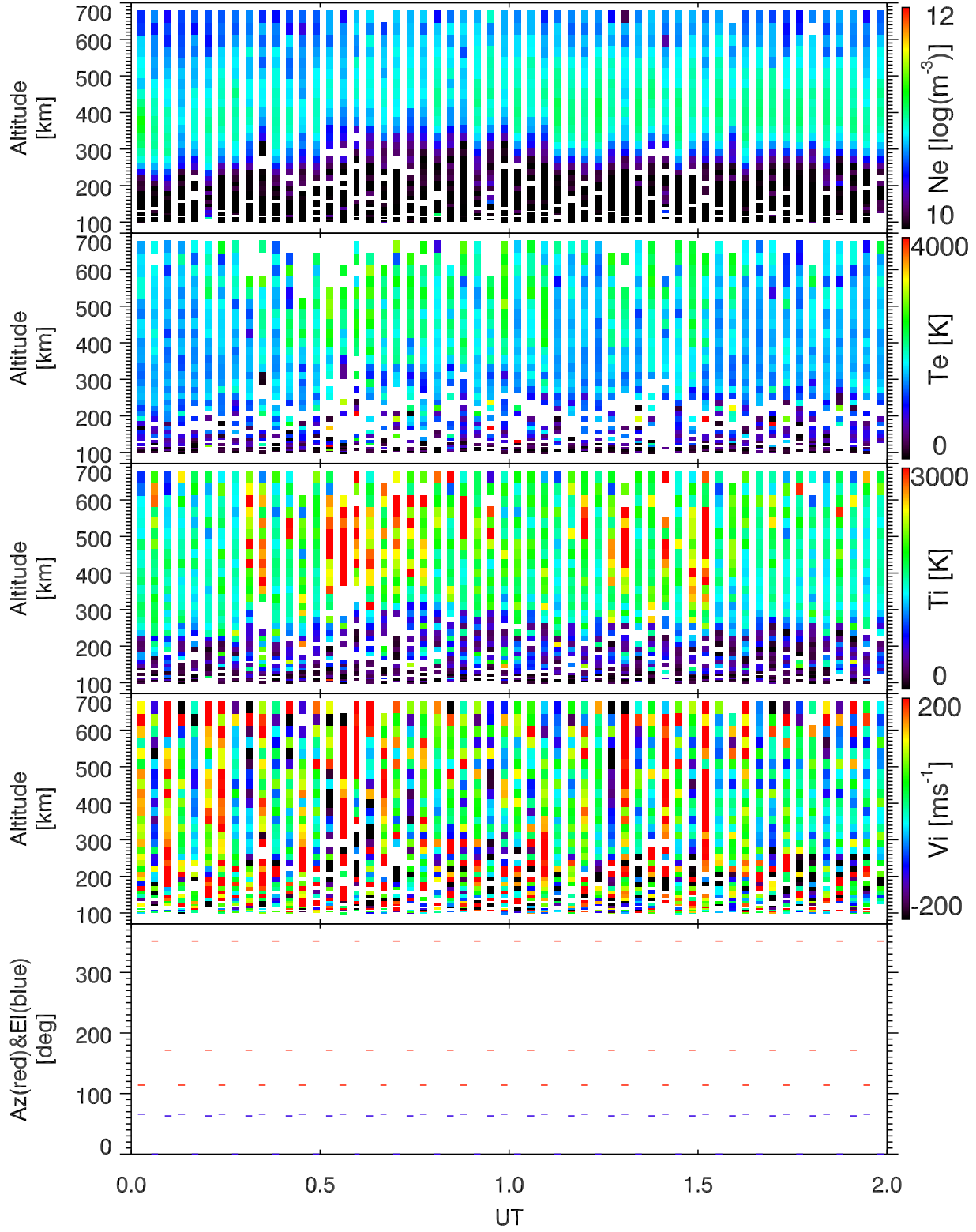
EISCAT 2002-10-17_00_02UT_tau0_ant@32m.
